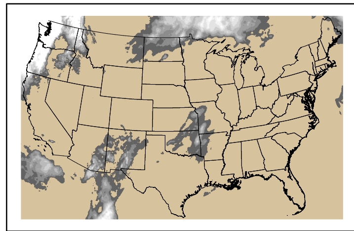
Precipitation p24m_202411200f144.bil
