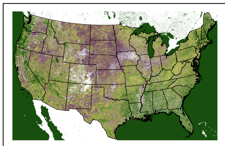
Greenness us24_309315wk_greenness.img
