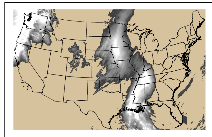
Precipitation p24m_202411200f048.bil
