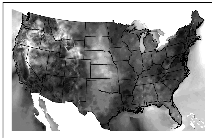
Wind Speed wspd20241113.bil
