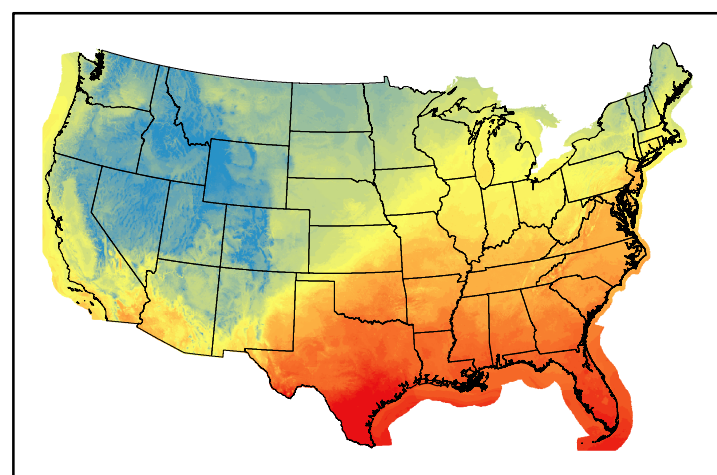
Dry Bulb Temp temp20241117.bil
