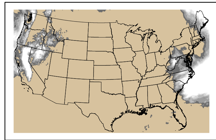
Precipitation p24m_202411200f096.bil
