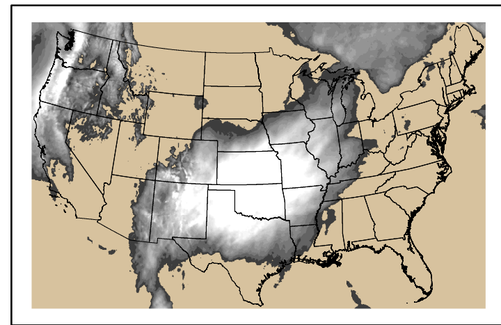
Precipitation p24m_202411200f168.bil
