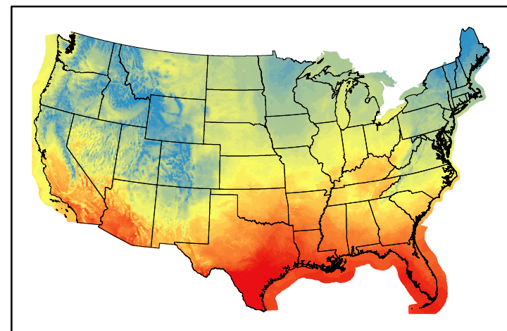
Dry Bulb Temp temp20241113.bil
