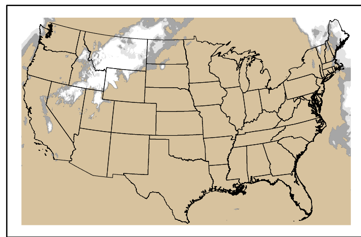
Precipitation p24m_202411200f120.bil
