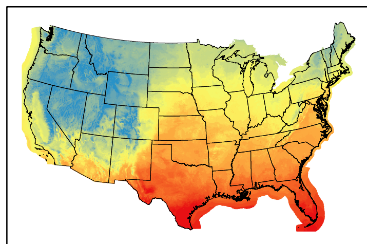
Dry Bulb Temp temp20241116.bil
