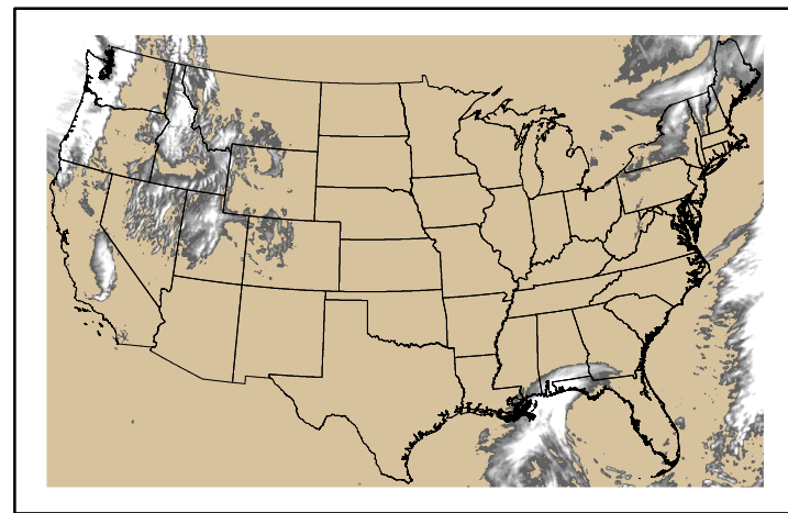
Precipitation p24m_202411200f024.bil
