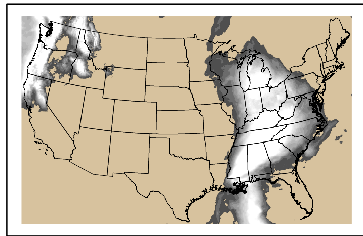
Precipitation p24m_202411200f072.bil
