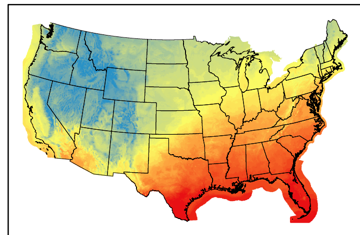
Dry Bulb Temp temp20241118.bil
