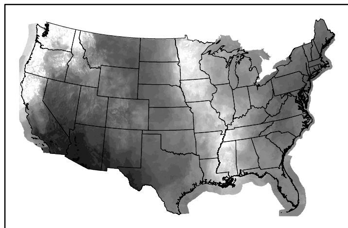
10hr Fuel Moisture mc10241113.bil
