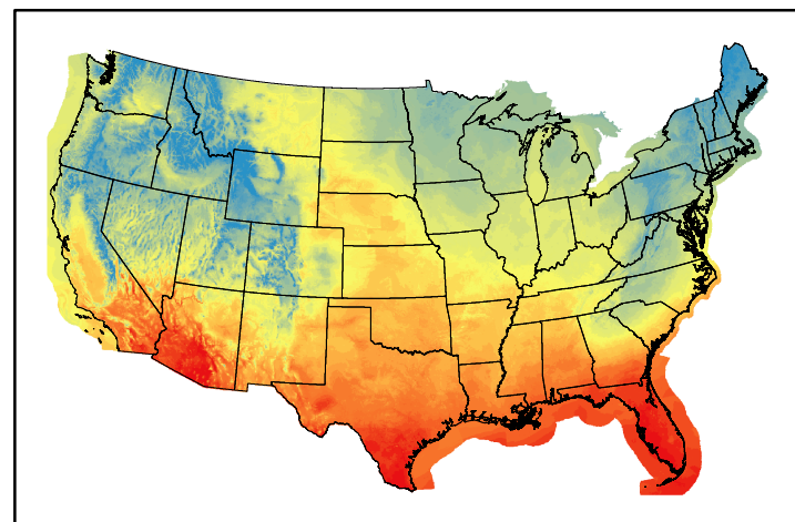
Dry Bulb Temp temp20241114.bil
