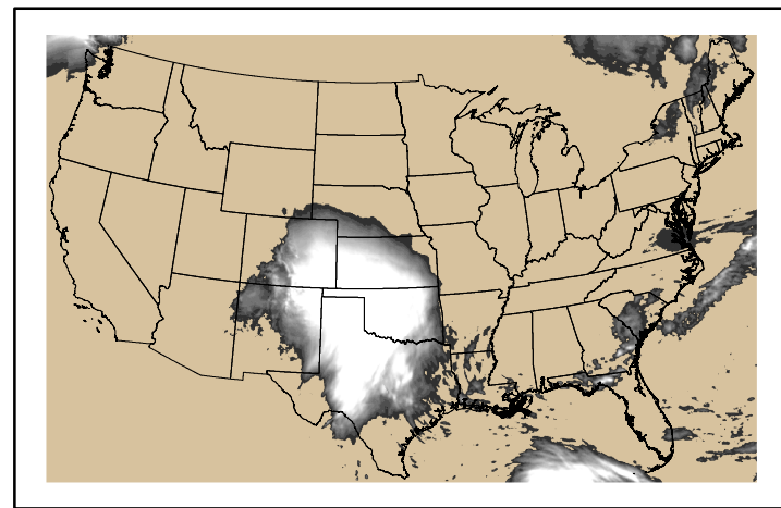
Precipitation p24m_2024110800f024.bil
