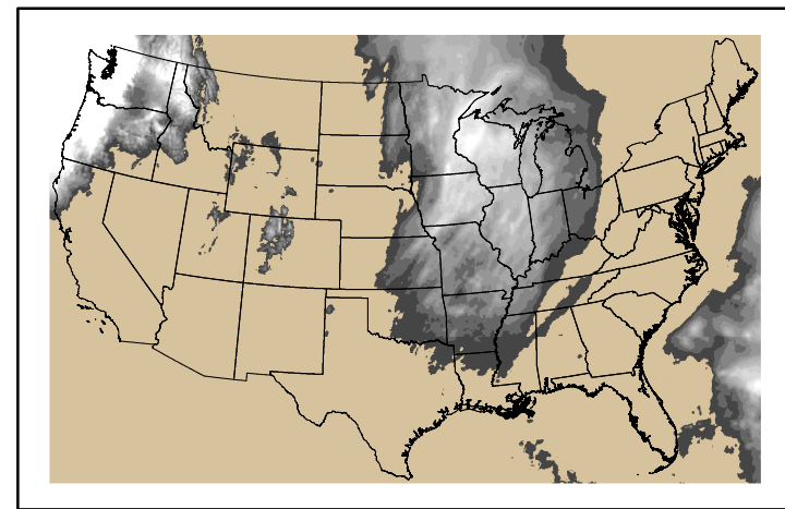
Precipitation p24m_2024110800f144.bil
