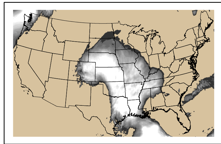
Precipitation p24m_2024110800f048.bil
