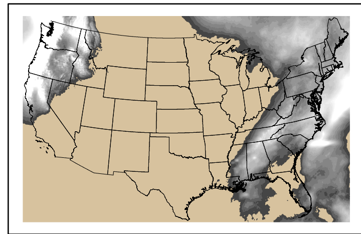
Precipitation p24m_2024110800f096.bil
