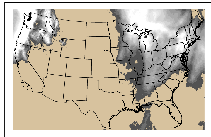
Precipitation p24m_2024110800f168.bil
