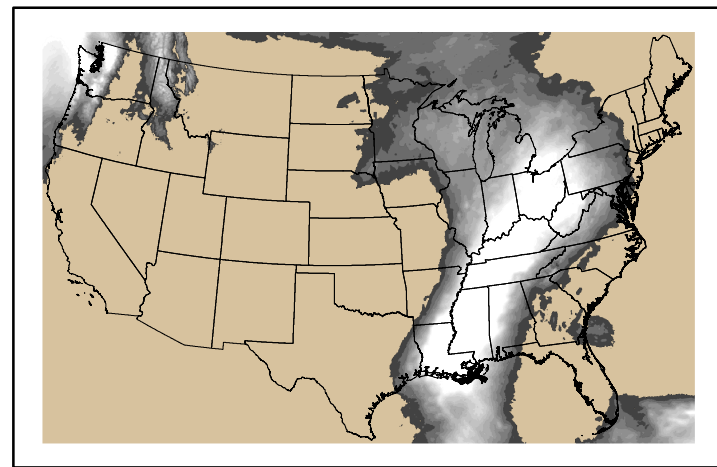
Precipitation p24m_2024110800f072.bil
