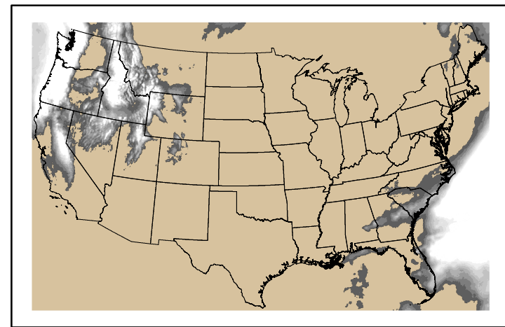
Precipitation p24m_2024110800f120.bil
