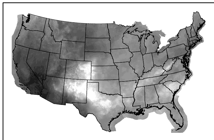
10hr Fuel Moisture mc10241107.bil
