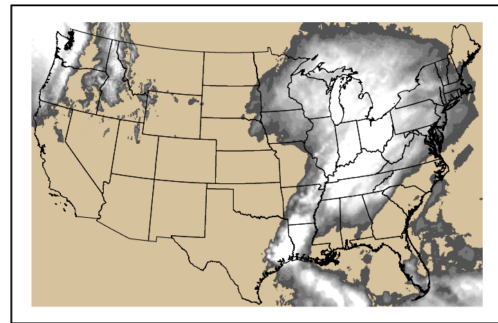
Precipitation p24m_2024110600f120.bil
