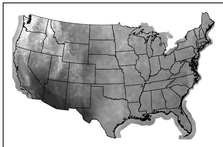
10hr Fuel Moisture mc10241112.bil
