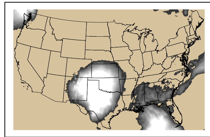
Precipitation p24m_2024110600f072.bil
