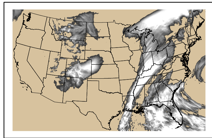
Precipitation p24m_2024110600f024.bil
