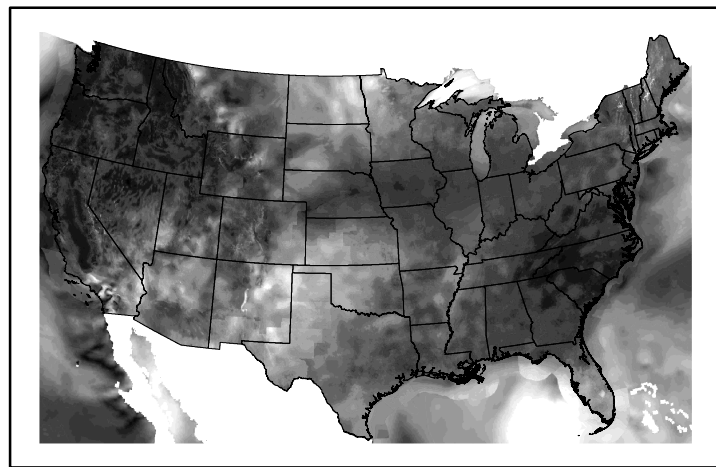
Wind Speed wspd20241107.bil
