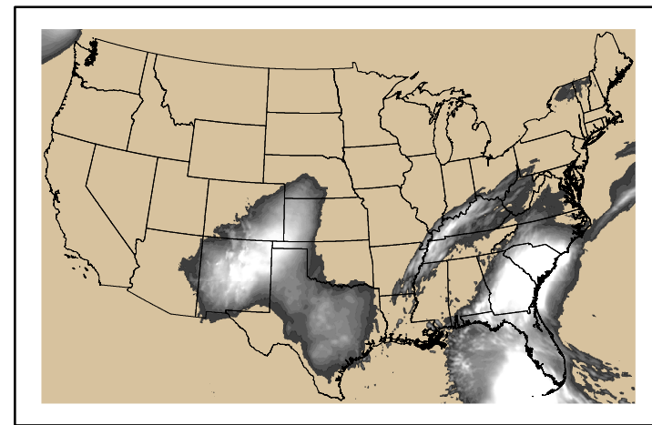
Precipitation p24m_2024110600f048.bil
