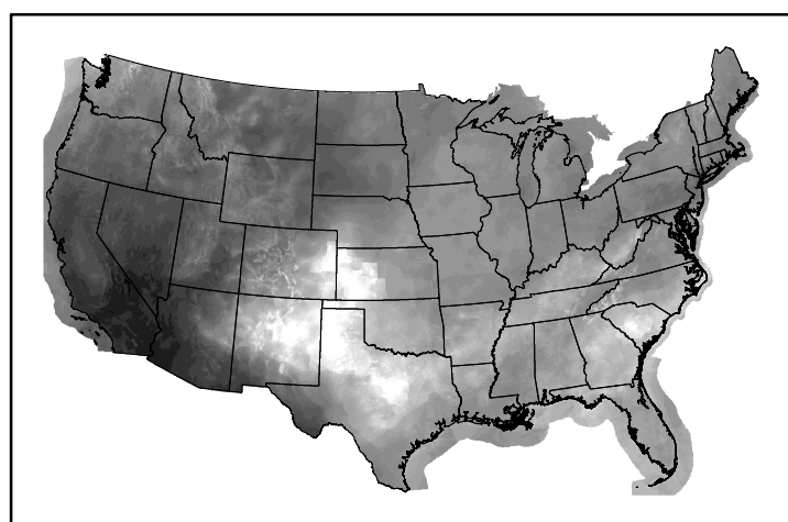
10hr Fuel Moisture mc10241107.bil
