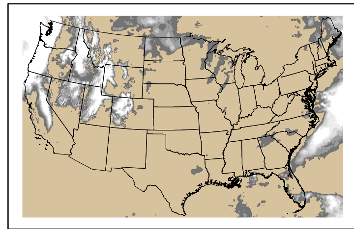
Precipitation p24m_2024110600f168.bil
