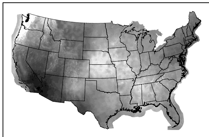
10hr Fuel Moisture mc10241109.bil
