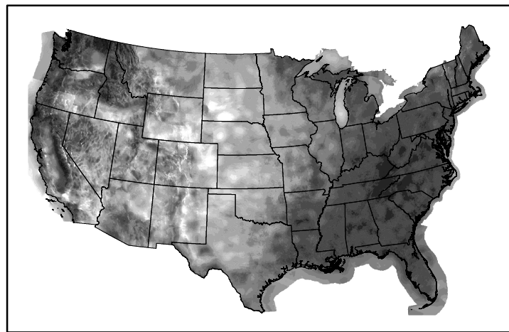
Wind Speed wspd20241112.bil
