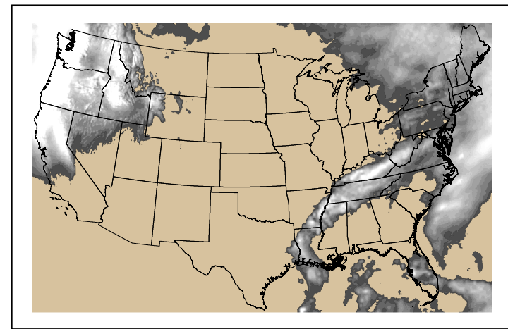
Precipitation p24m_2024110600f144.bil
