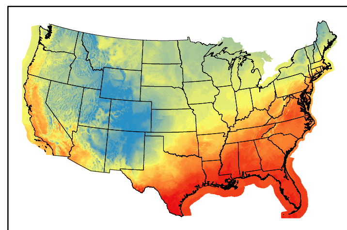
Dry Bulb Temp temp20241107.bil
