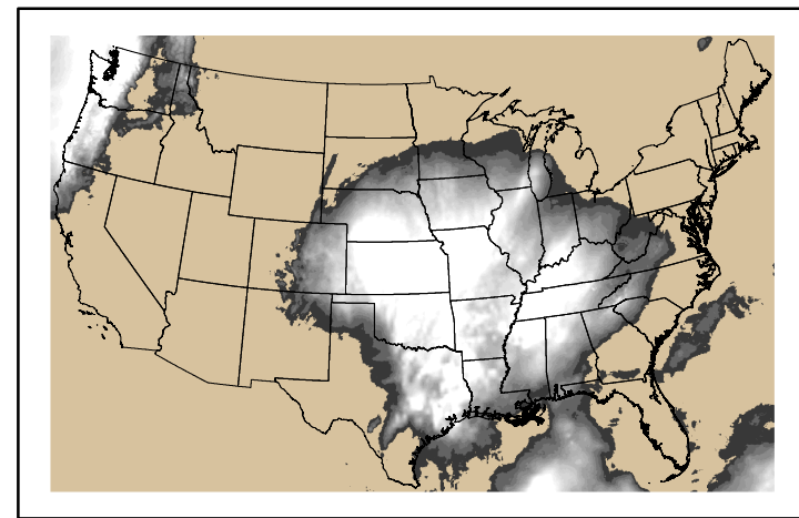
Precipitation p24m_2024110600f096.bil
