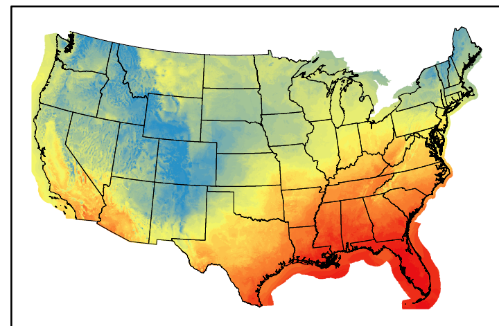
Dry Bulb Temp temp20241109.bil
