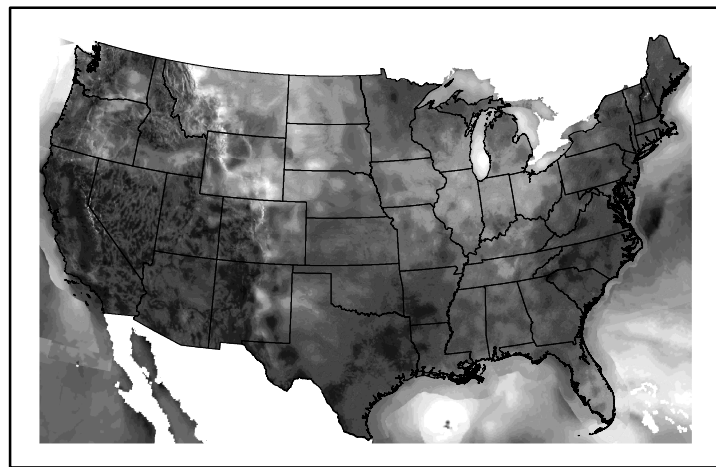
Wind Speed wspd20241110.bil
