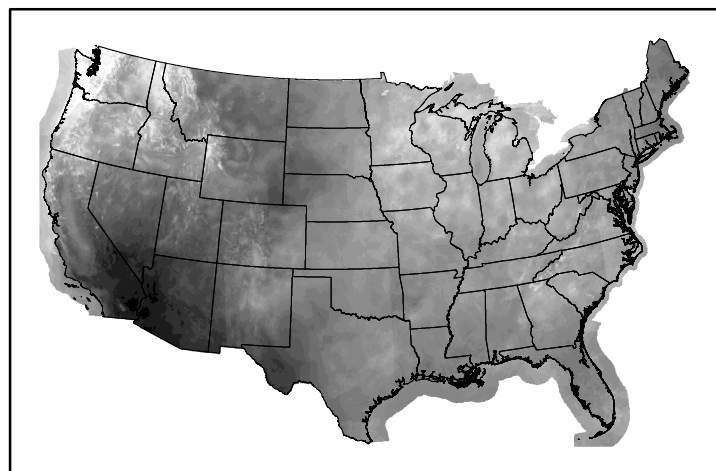
10hr Fuel Moisture mc10241110.bil
