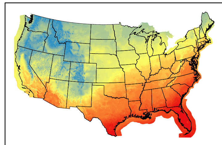
Dry Bulb Temp temp20241111.bil
