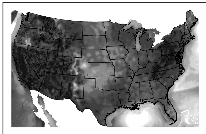
Wind Speed wspd20241109.bil
