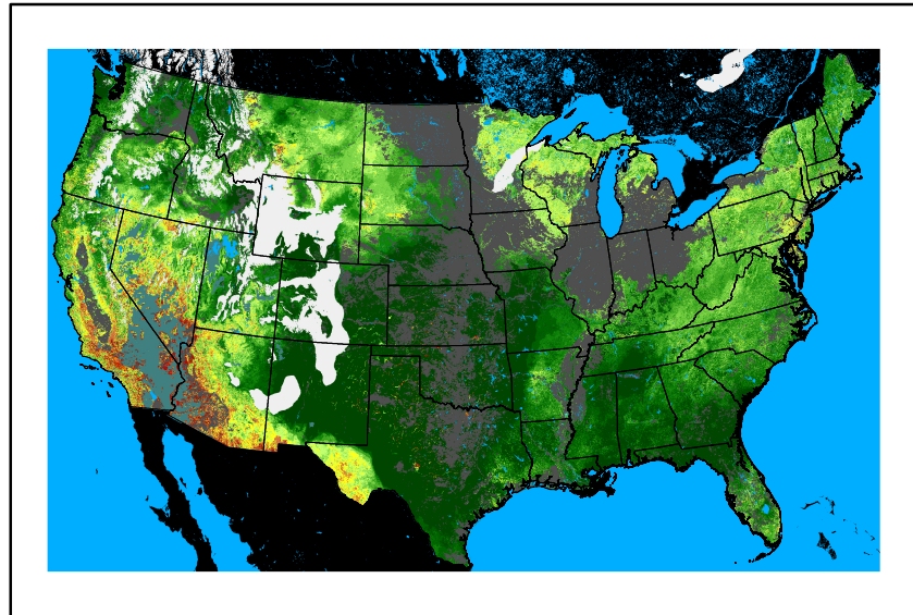
WFPI fp241108.bil
