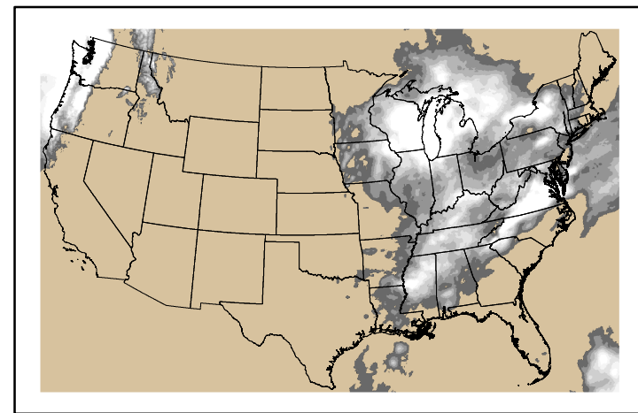
Precipitation p24m_2024110400f168.bil
