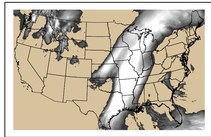
Precipitation p24m_2024110400f048.bil
