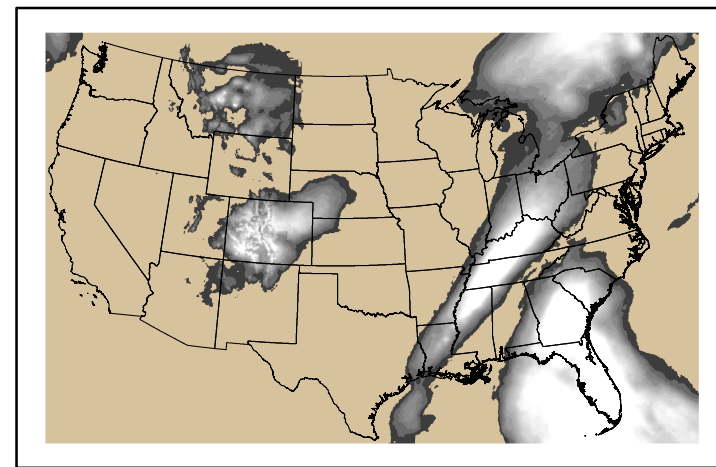
Precipitation p24m_2024110400f072.bil
