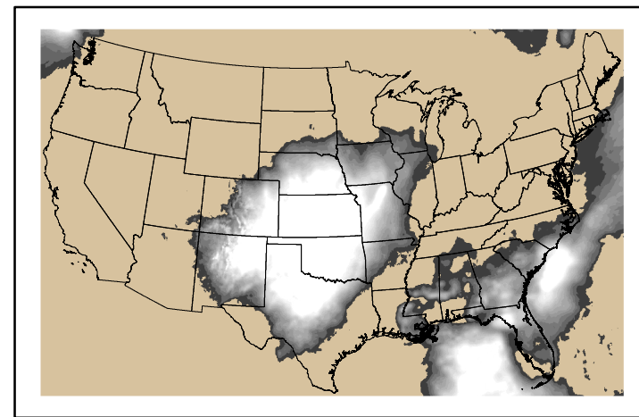
Precipitation p24m_2024110400f120.bil
