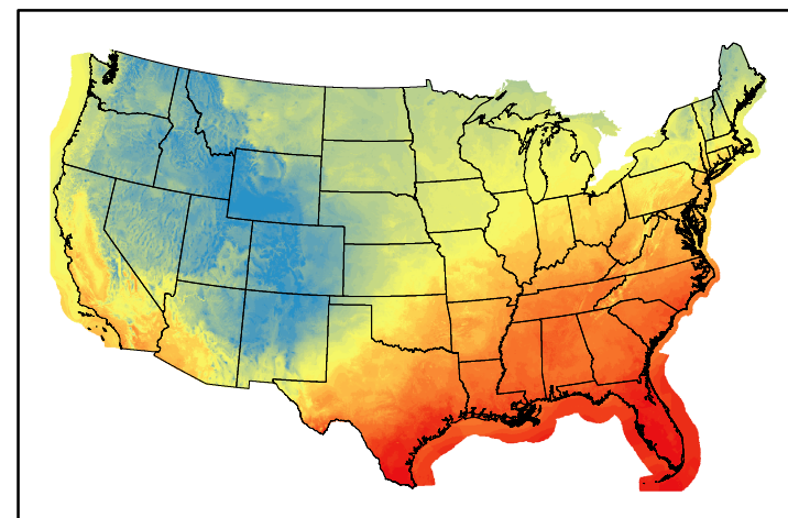
Dry Bulb Temp temp20241108.bil
