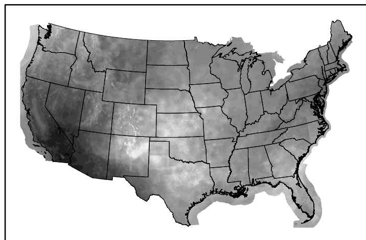
10hr Fuel Moisture mc10241108.bil
