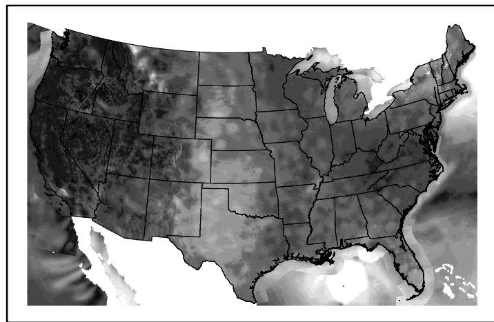
Wind Speed wspd20241108.bil
