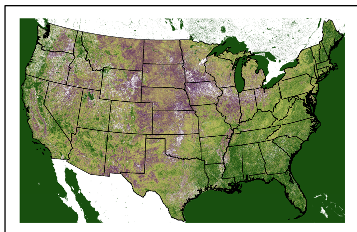
Greenness us24_302308wk_greenness.img
