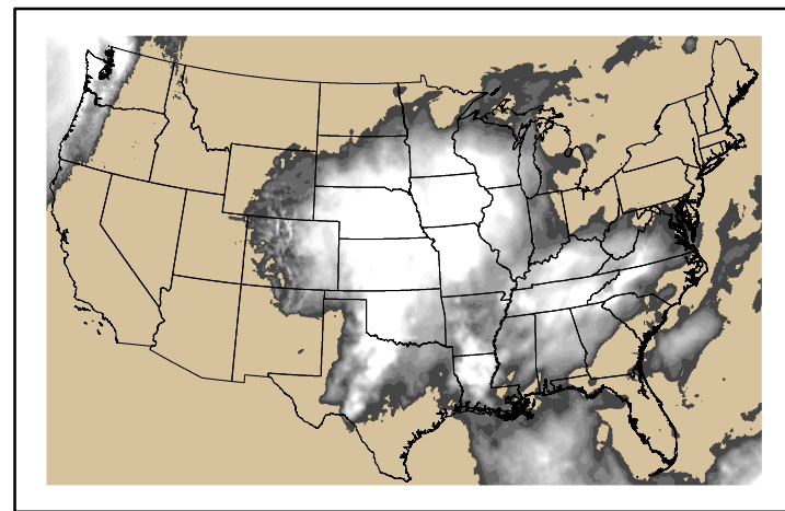
Precipitation p24m_2024110400f144.bil
