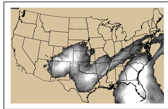
Precipitation p24m_2024110400f096.bil
