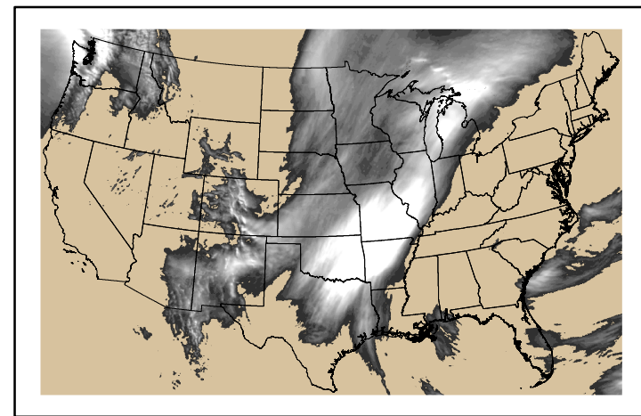
Precipitation p24m_2024110400f024.bil
