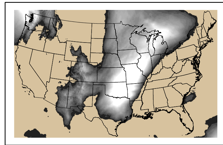
Precipitation p24m_2024110200f072.bil
