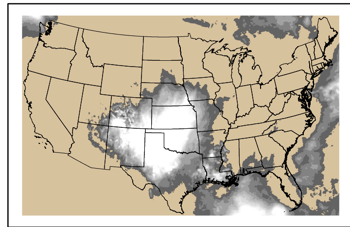
Precipitation p24m_2024110200f168.bil
