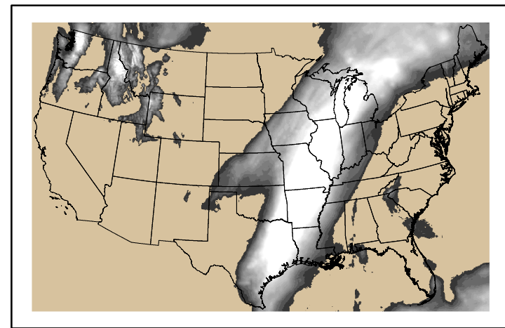
Precipitation p24m_2024110200f096.bil
