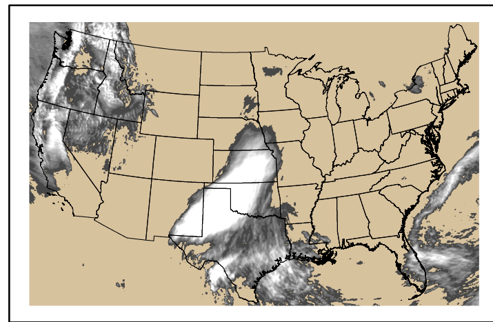
Precipitation p24m_2024110200f024.bil
