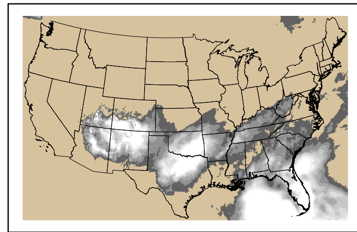
Precipitation p24m_2024110200f144.bil
