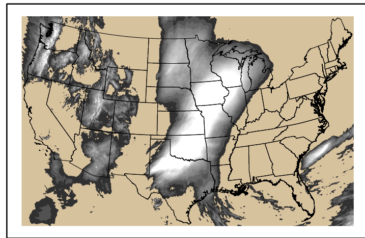
Precipitation p24m_2024110200f048.bil
