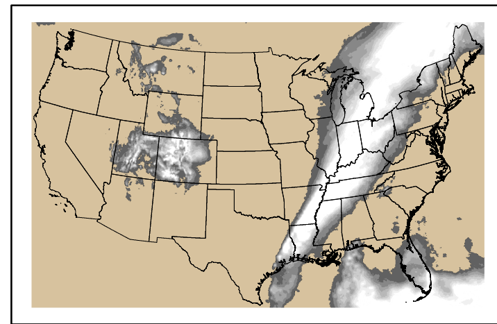
Precipitation p24m_2024110200f120.bil
