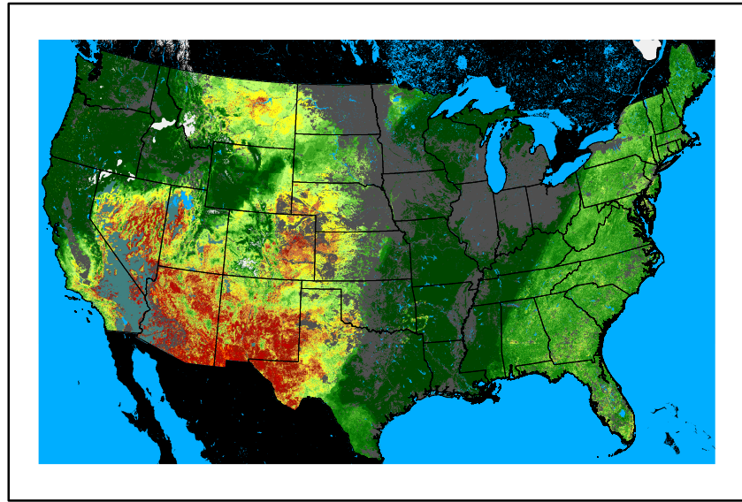
WFPI fp241031.bil
