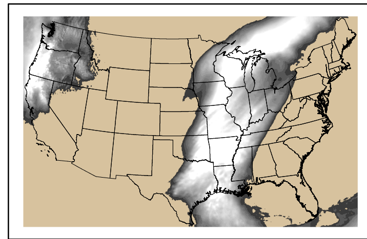
Precipitation p24m_2024102900f072.bil
