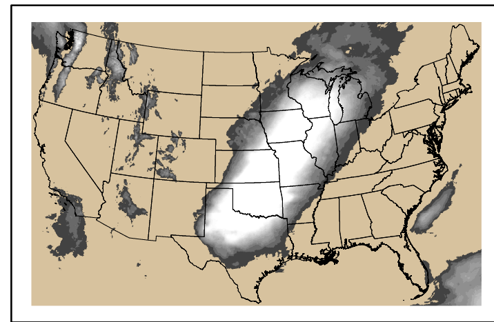
Precipitation p24m_2024102900f144.bil
