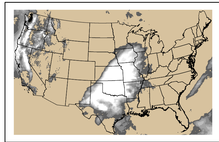
Precipitation p24m_2024102700f168.bil
