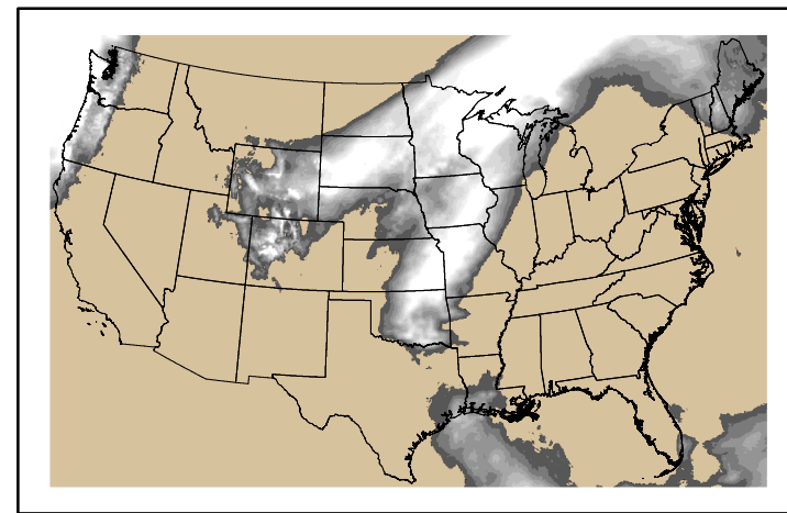
Precipitation p24m_2024102700f096.bil
