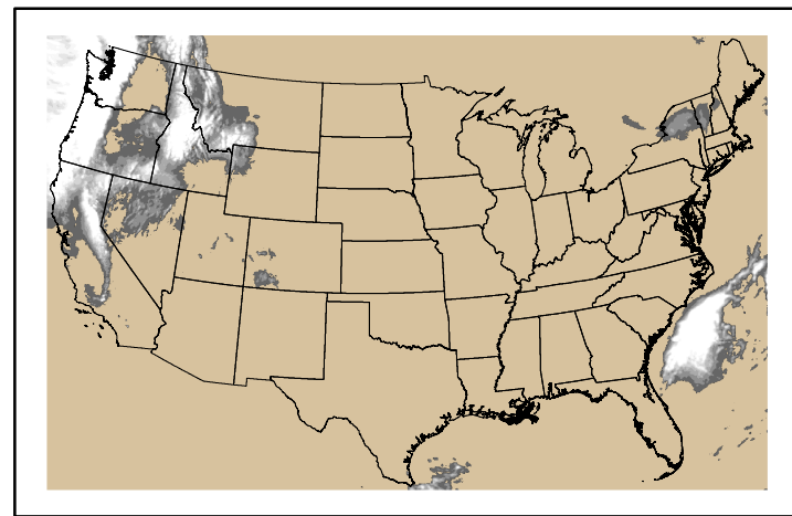
Precipitation p24m_2024102700f048.bil
