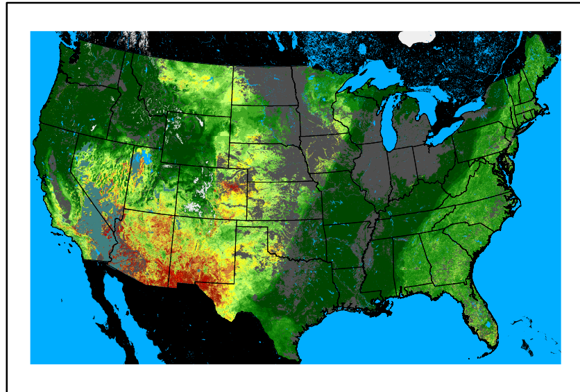
WFPI fp241031.bil
