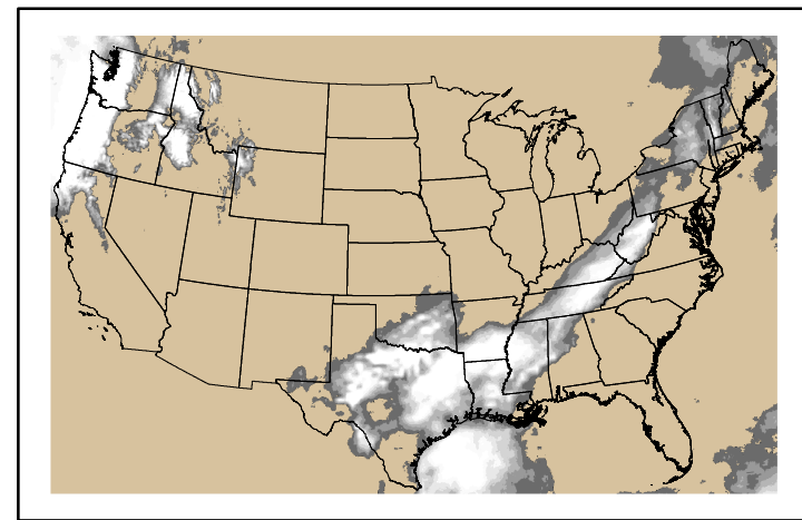
Precipitation p24m_2024102700f144.bil
