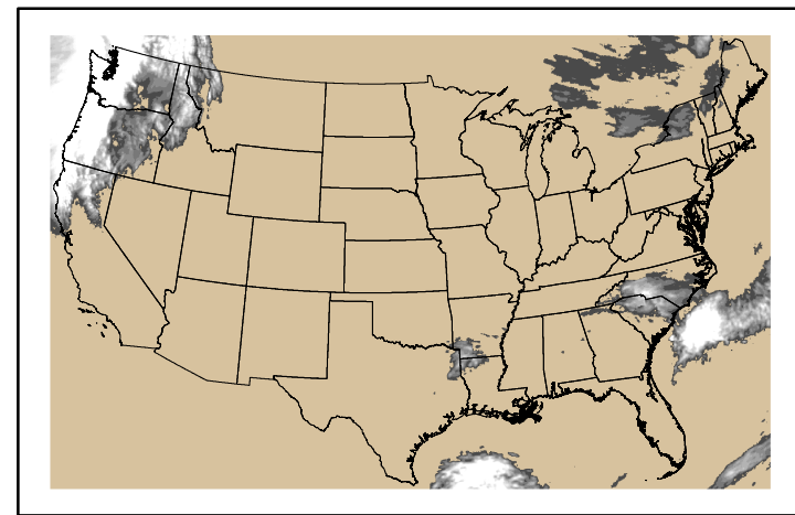
Precipitation p24m_2024102700f024.bil
