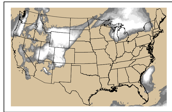
Precipitation p24m_2024102700f072.bil
