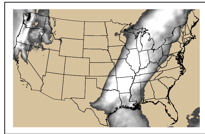
Precipitation p24m_2024102700f120.bil
