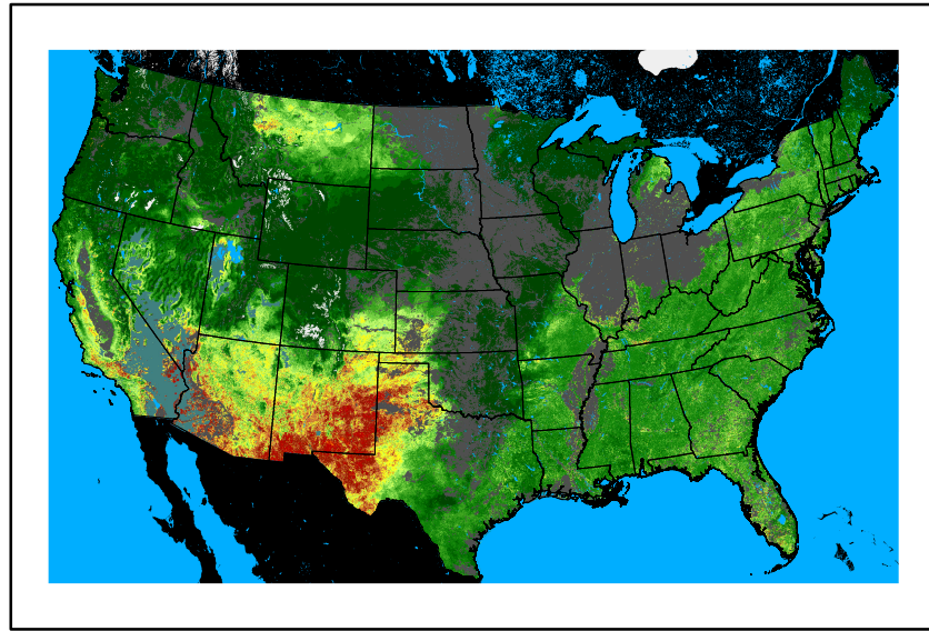
WFPI fp241030.bil
