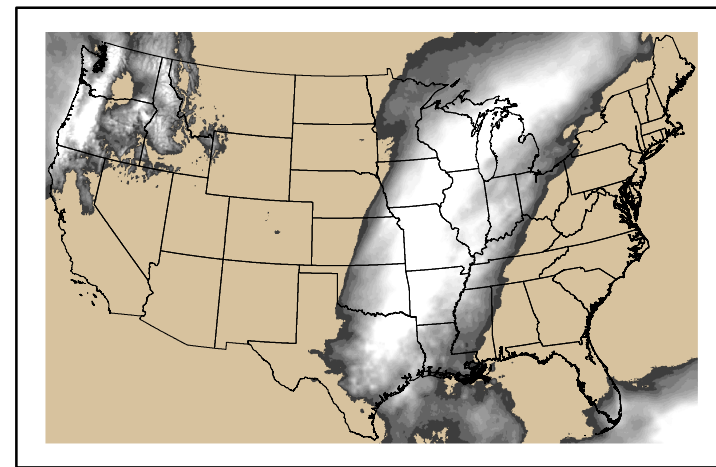
Precipitation p24m_2024102600f144.bil
