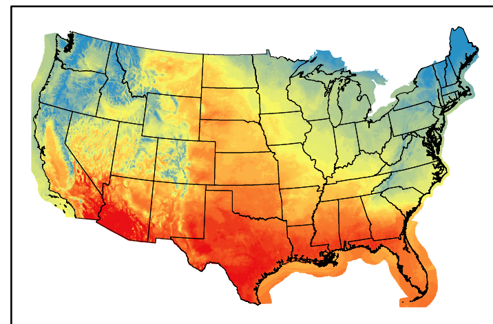
Dry Bulb Temp temp20241027.bil
