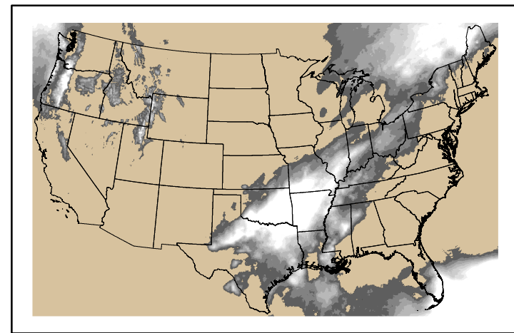
Precipitation p24m_2024102600f168.bil
