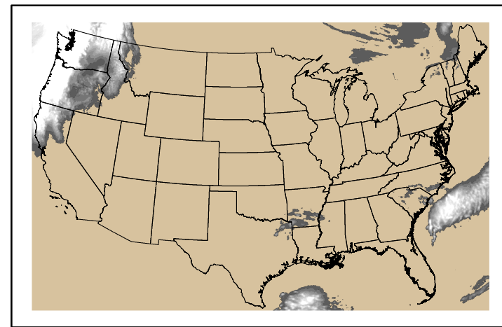
Precipitation p24m_2024102600f048.bil
