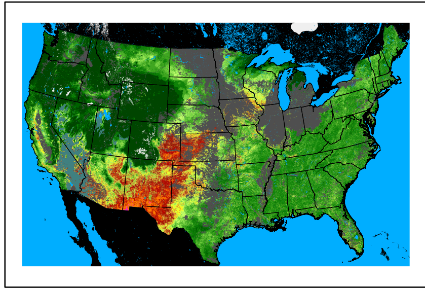
WFPI fp241029.bil
