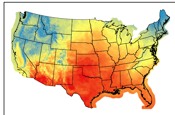
Dry Bulb Temp temp20241028.bil
