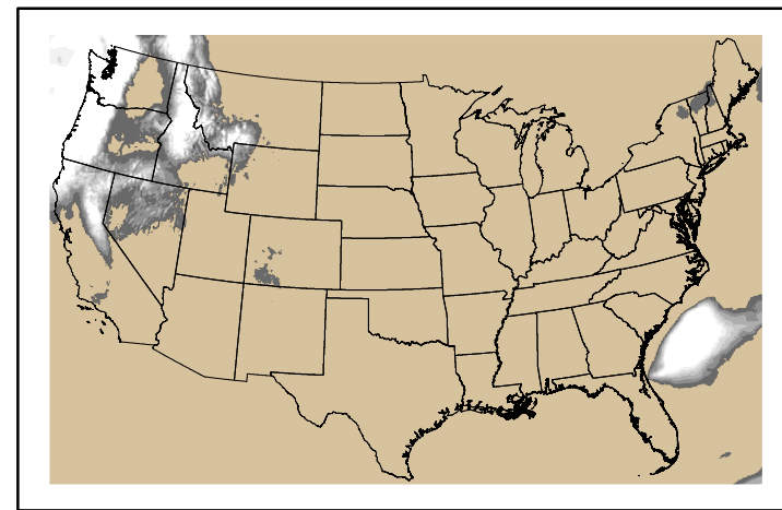
Precipitation p24m_2024102600f072.bil
