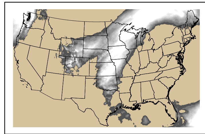
Precipitation p24m_2024102600f120.bil
