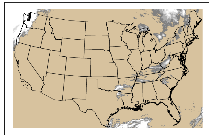
Precipitation p24m_2024102600f024.bil
