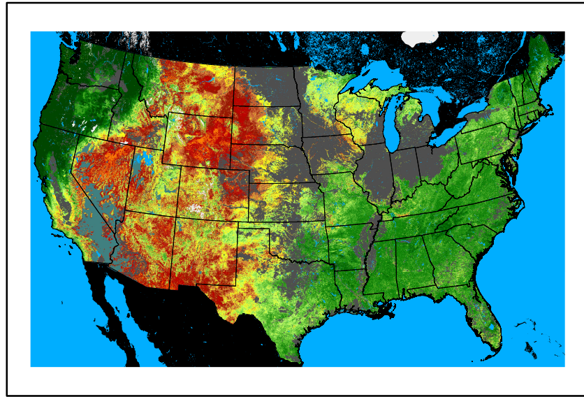
WFPI fp241027.bil
