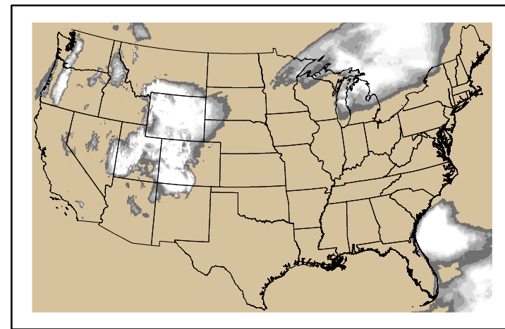
Precipitation p24m_2024102600f096.bil
