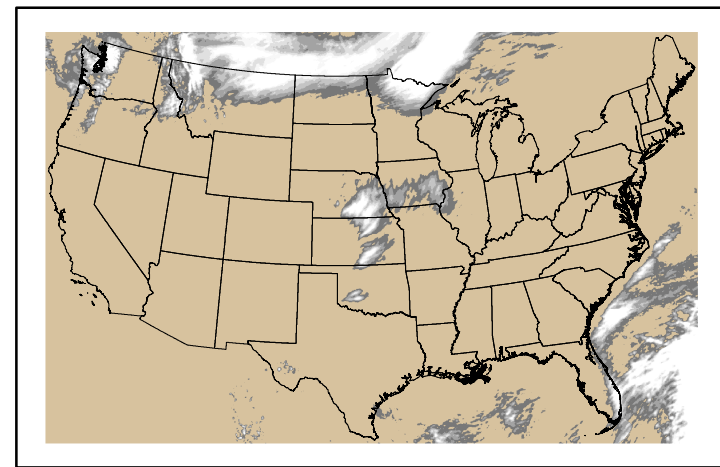
Precipitation p24m_2024102200f024.bil
