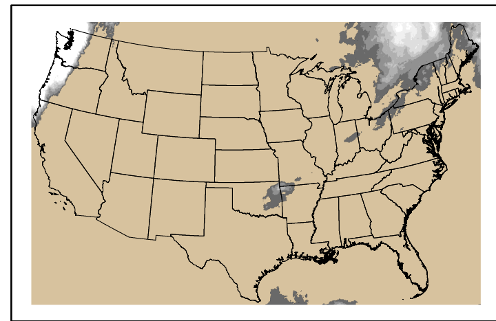
Precipitation p24m_2024102200f120.bil
