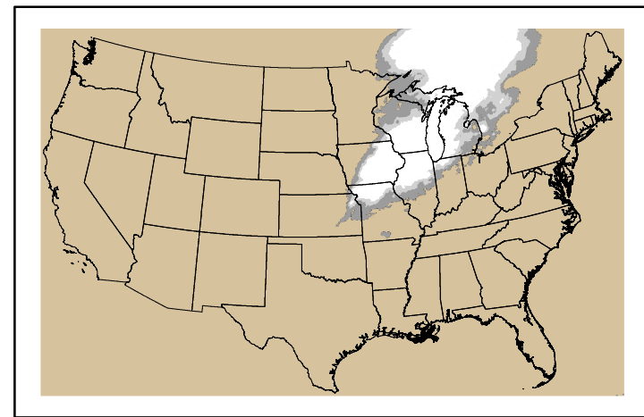
Precipitation p24m_2024102200f096.bil
