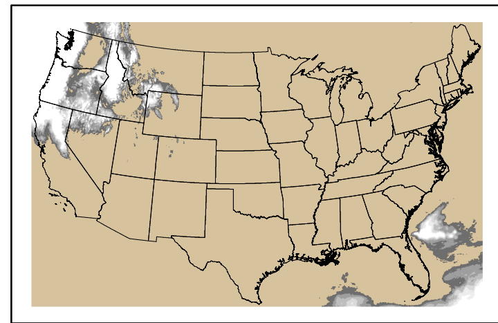
Precipitation p24m_2024102200f168.bil
