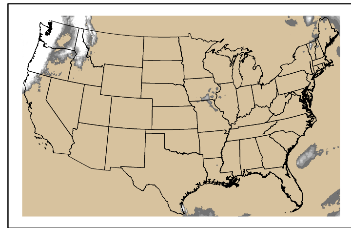
Precipitation p24m_2024102200f144.bil
