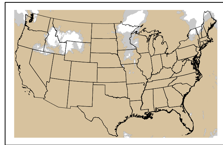
Precipitation p24m_2024102200f072.bil
