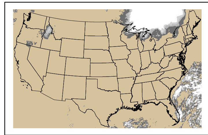
Precipitation p24m_2024102200f048.bil
