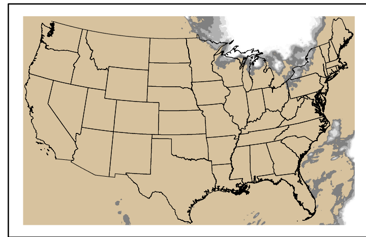
Precipitation p24m_2024102100f072.bil
