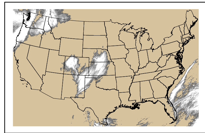
Precipitation p24m_2024102100f024.bil
