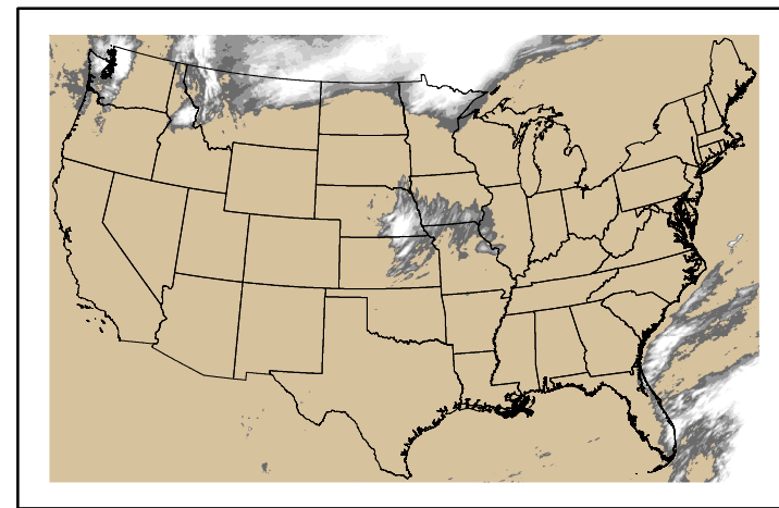
Precipitation p24m_2024102100f048.bil
