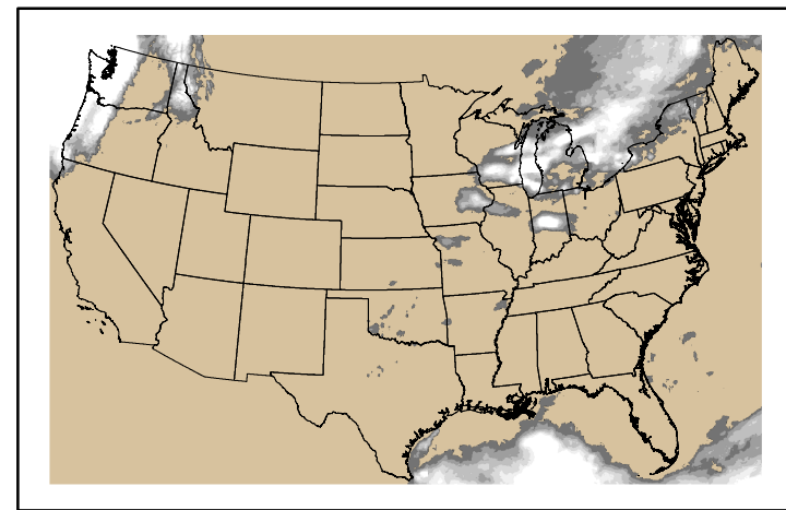
Precipitation p24m_2024102100f168.bil
