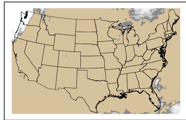
Precipitation p24m_2024102100f144.bil
