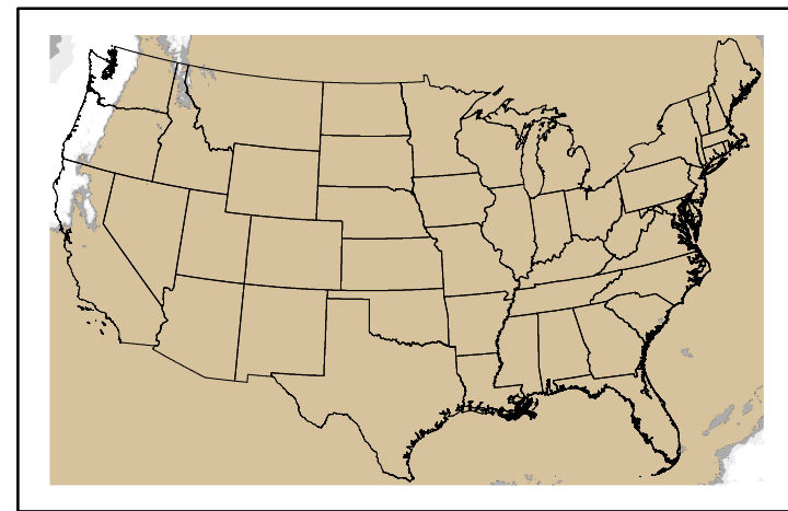
Precipitation p24m_2024102100f120.bil
