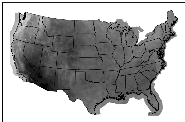
10hr Fuel Moisture mc10241025.bil
