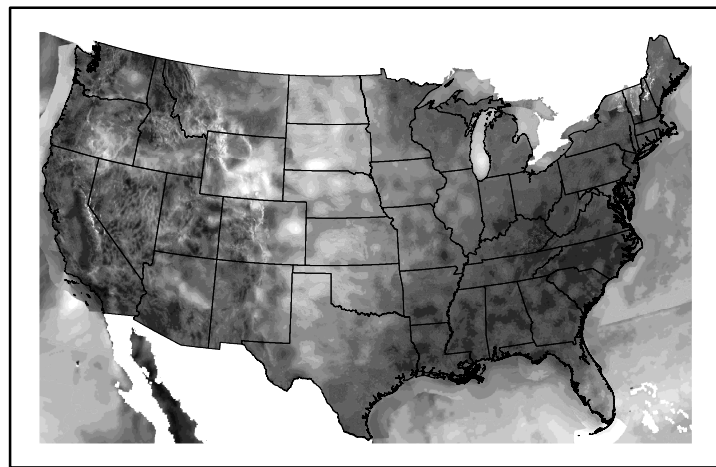
Wind Speed wspd20241025.bil
