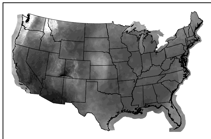
10hr Fuel Moisture mc10241021.bil
