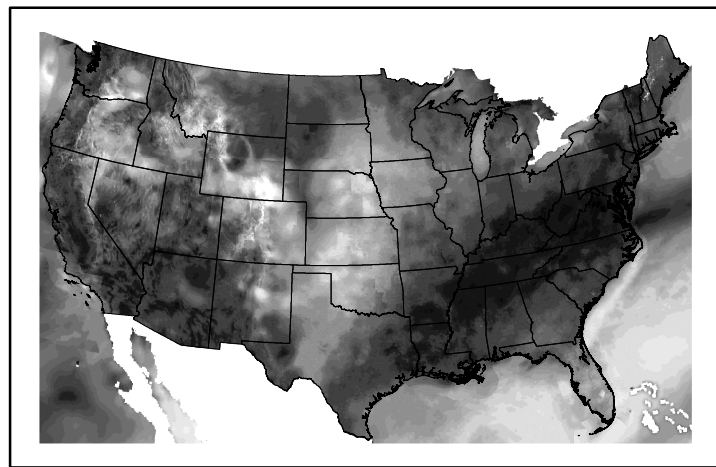
Wind Speed wspd20241021.bil
