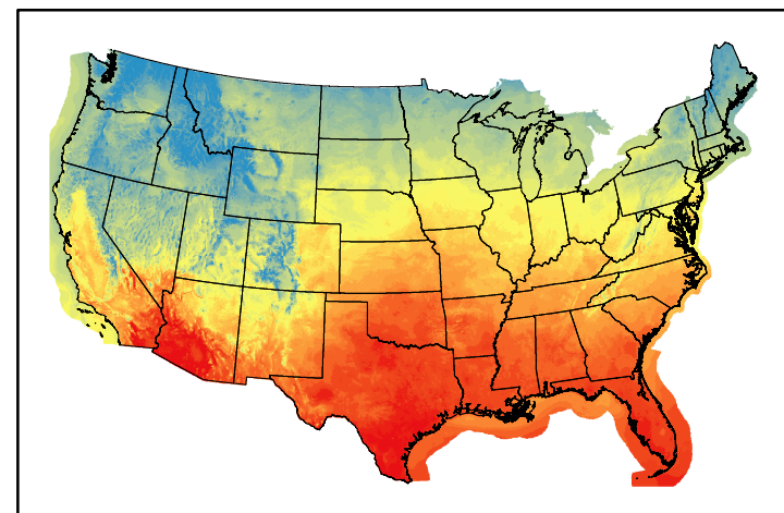
Dry Bulb Temp temp20241026.bil
