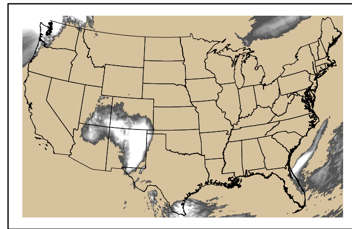
Precipitation p24m_2024102000f024.bil
