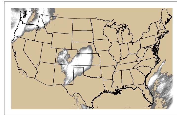
Precipitation p24m_2024102000f048.bil
