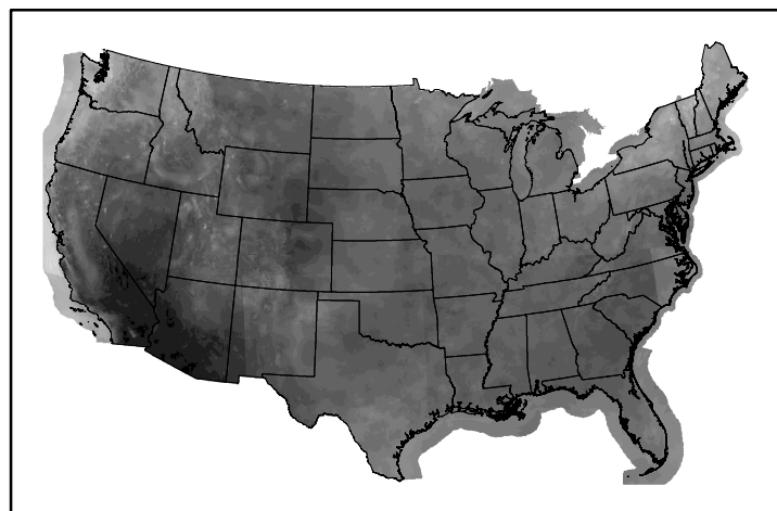
10hr Fuel Moisture mc10241024.bil
