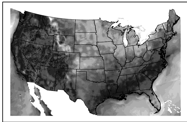
Wind Speed wspd20241023.bil
