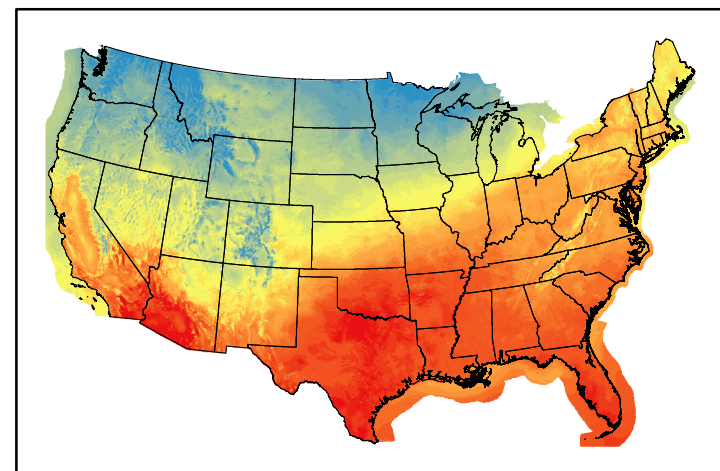
Dry Bulb Temp temp20241023.bil
