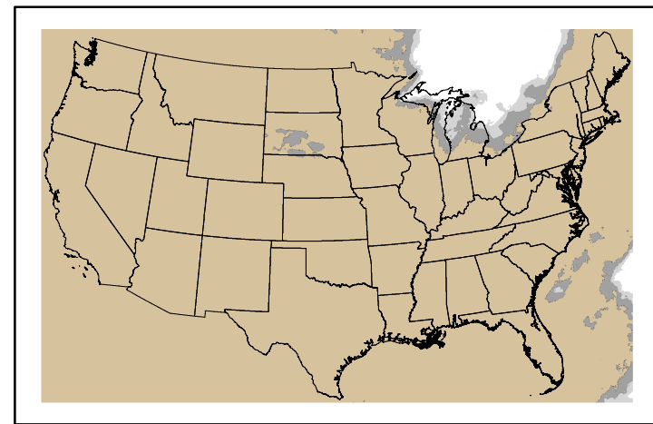
Precipitation p24m_2024102000f096.bil
