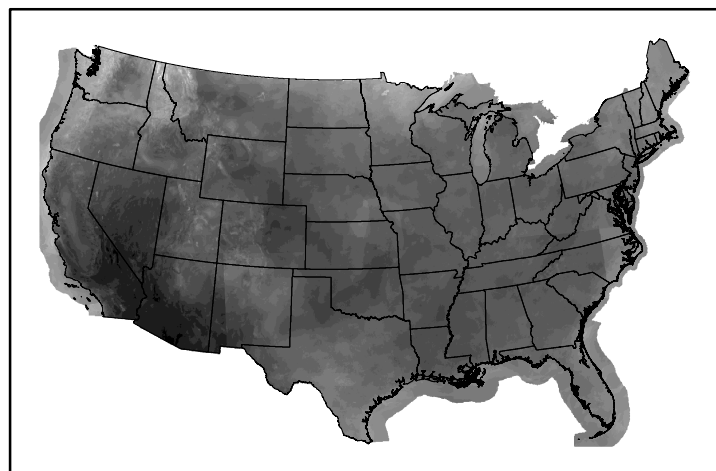
10hr Fuel Moisture mc10241022.bil
