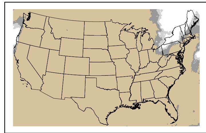
Precipitation p24m_2024102000f120.bil
