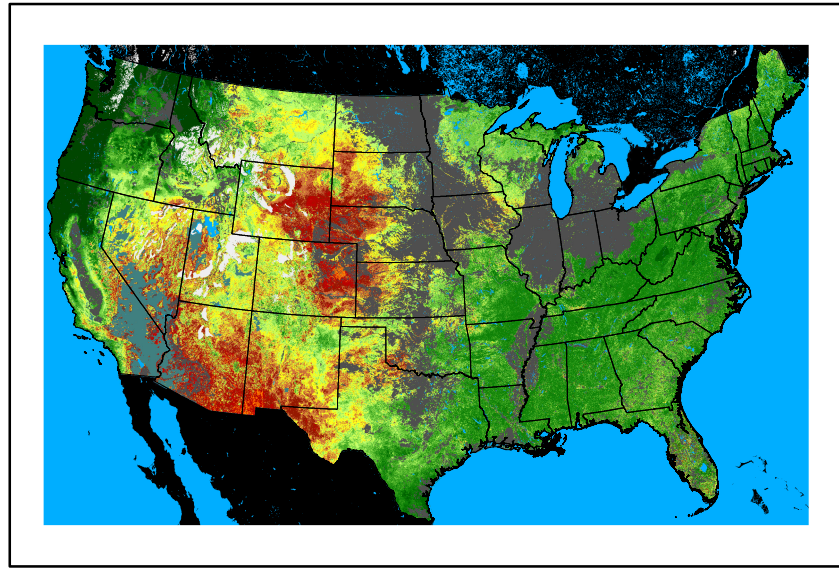
WFPI fp241026.bil
