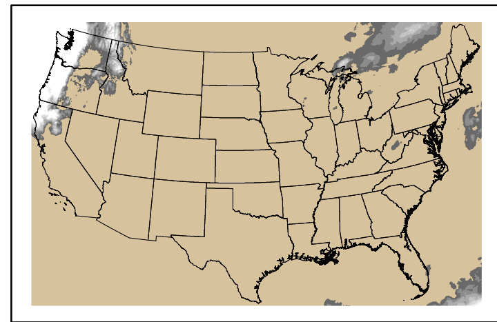
Precipitation p24m_2024102000f168.bil
