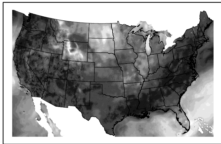
Wind Speed wspd20241022.bil
