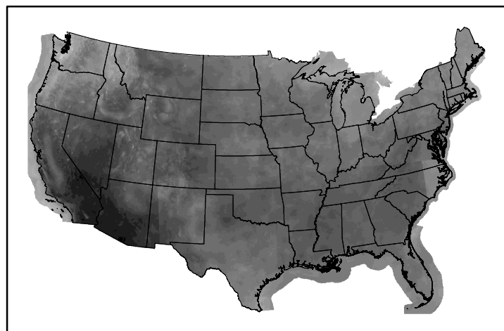
10hr Fuel Moisture mc10241023.bil
