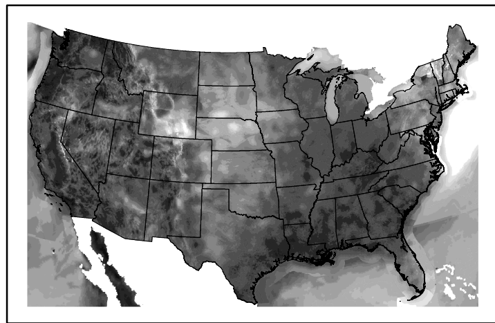
Wind Speed wspd20241024.bil
