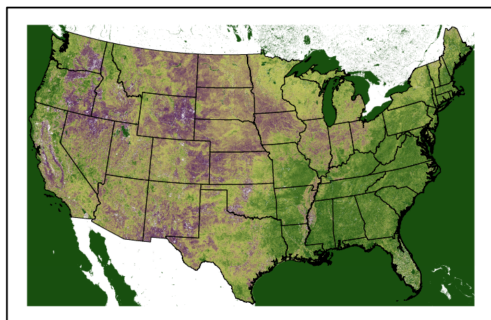
Greenness us24_281287wk_greenness.img
