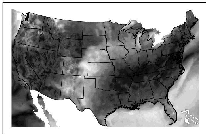
Wind Speed wspd20241020.bil
