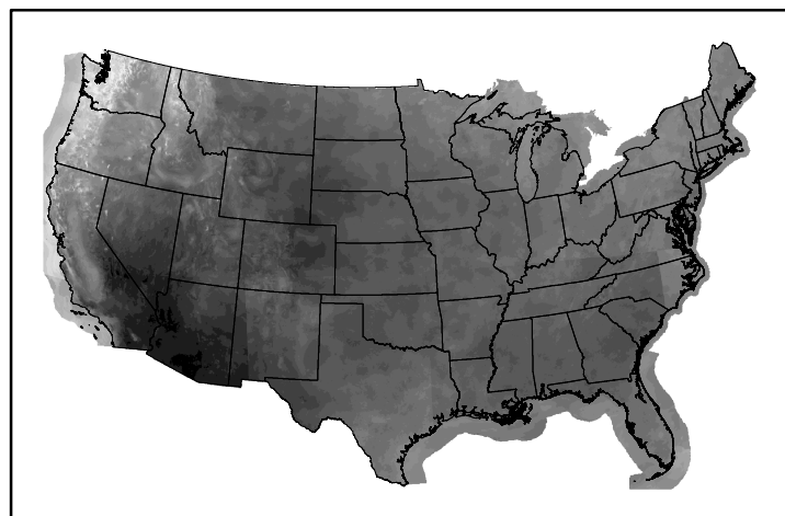
10hr Fuel Moisture mc10241026.bil
