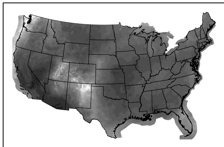
10hr Fuel Moisture mc10241020.bil
