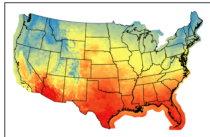
Dry Bulb Temp temp20241025.bil
