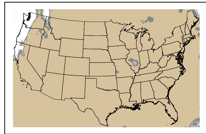
Precipitation p24m_2024102000f144.bil
