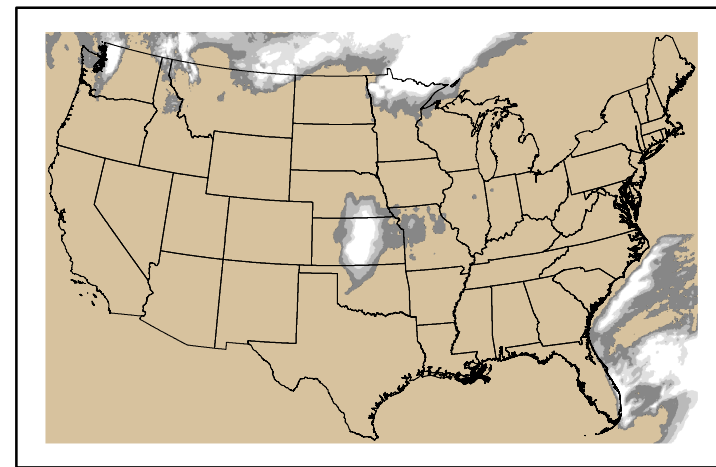
Precipitation p24m_2024102000f072.bil
