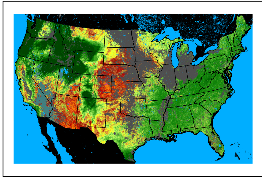
WFPI fp241017.bil
