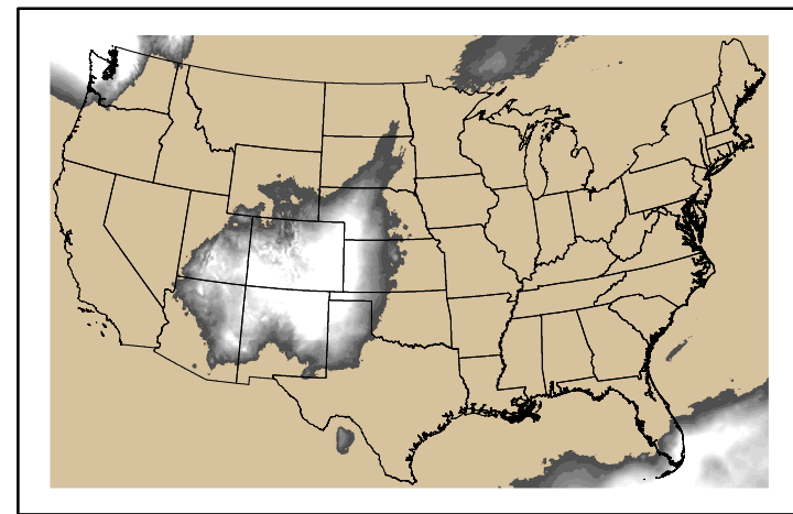
Precipitation p24m_2024101600f096.bil
