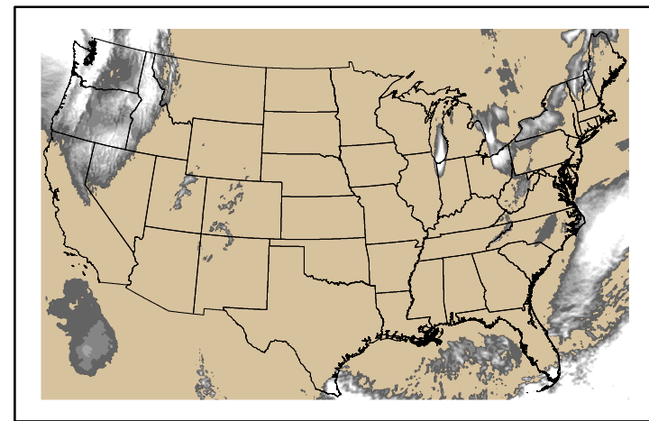
Precipitation p24m_2024101600f024.bil
