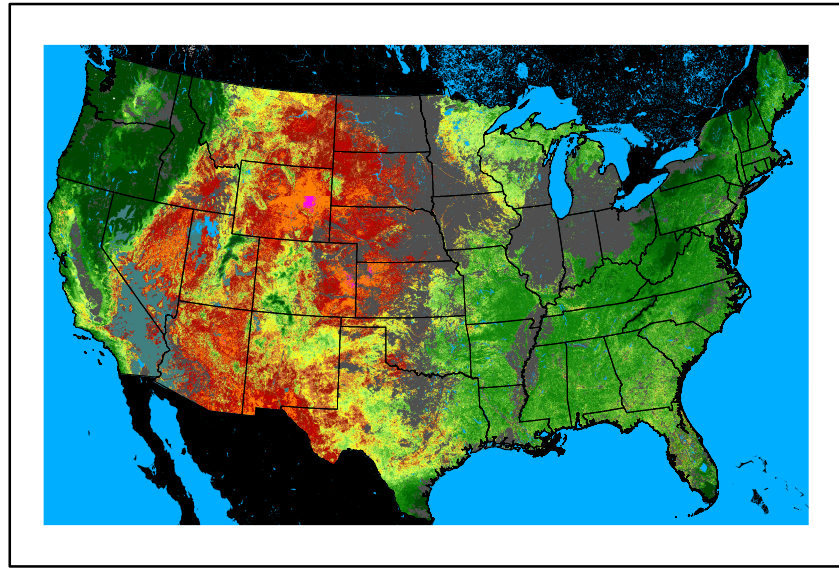
WFPI fp241016.bil
