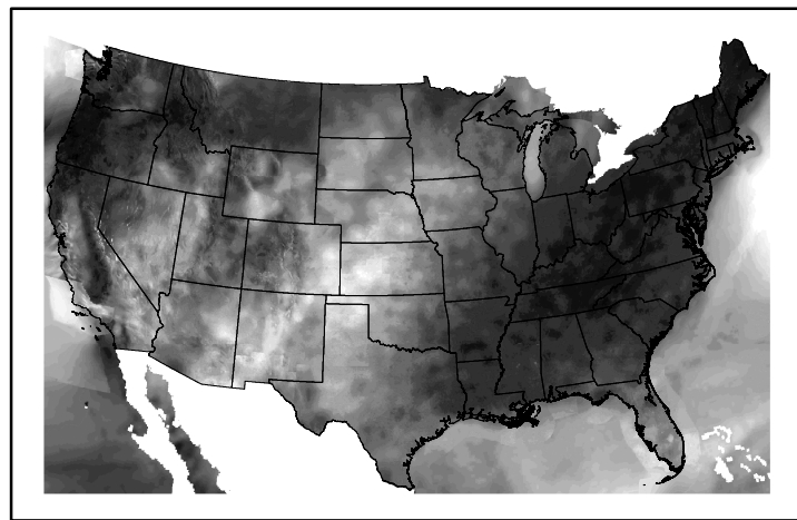
Wind Speed wspd20241018.bil
