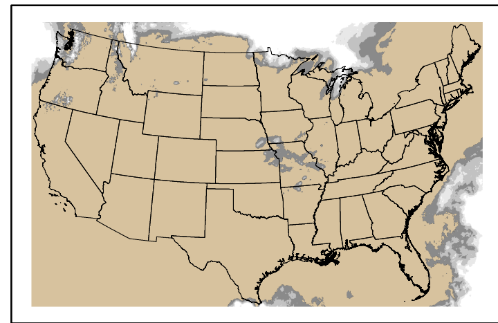
Precipitation p24m_2024101600f168.bil
