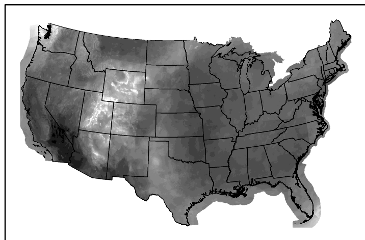
10hr Fuel Moisture mc10241018.bil
