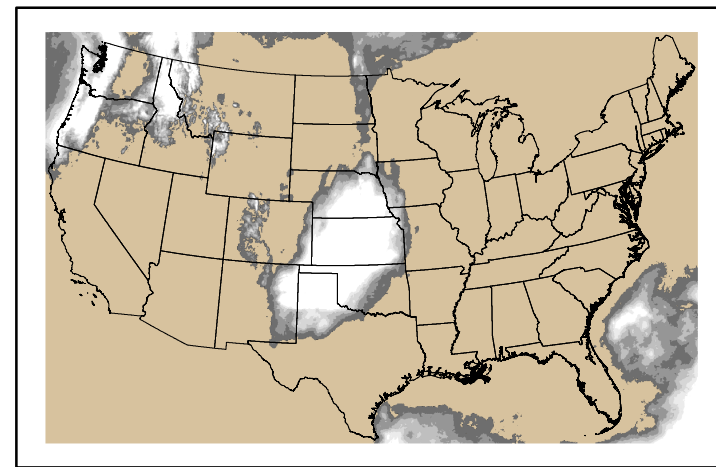
Precipitation p24m_2024101600f144.bil
