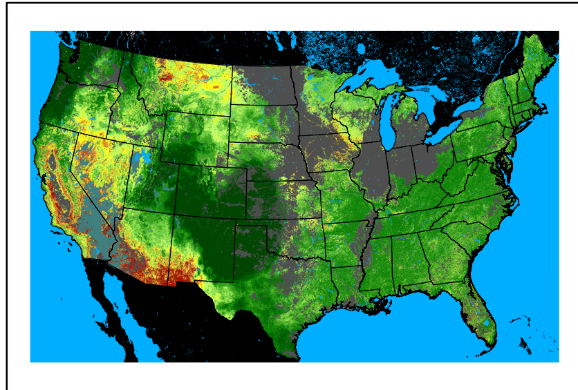
WFPI fp241020.bil
