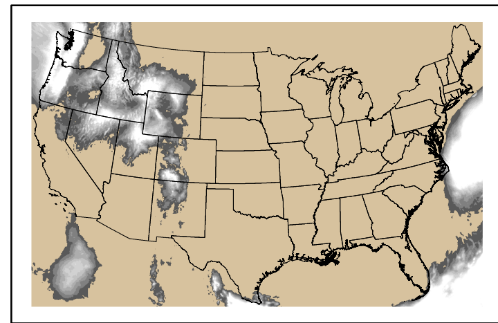
Precipitation p24m_2024101600f048.bil
