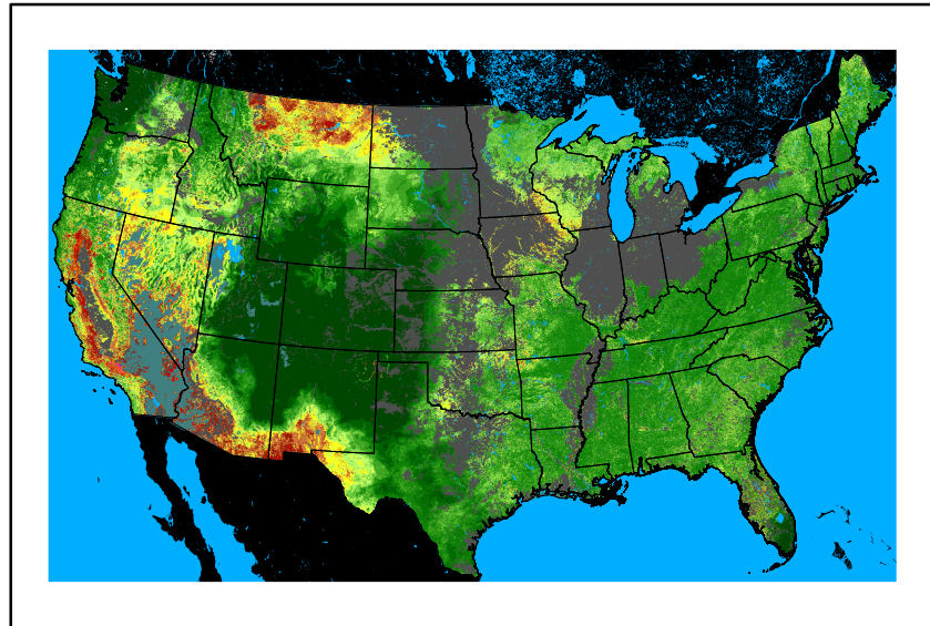
WFPI fp241019.bil
