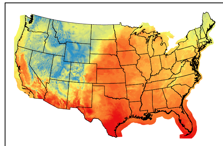
Dry Bulb Temp temp20241018.bil
