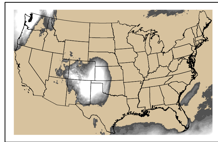
Precipitation p24m_2024101600f120.bil
