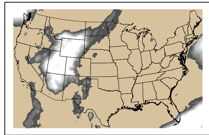
Precipitation p24m_2024101600f072.bil
