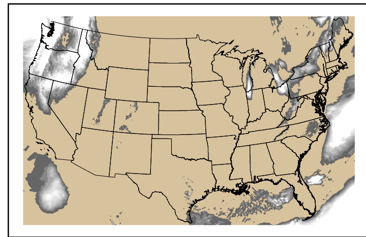
Precipitation p24m_2024101500f048.bil
