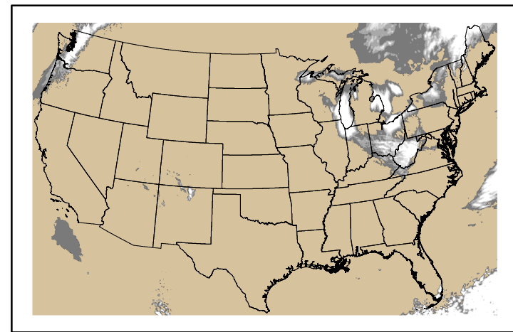
Precipitation p24m_2024101500f024.bil
