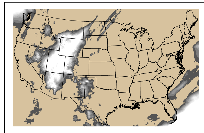
Precipitation p24m_2024101500f096.bil
