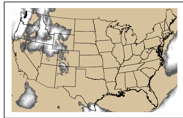
Precipitation p24m_2024101500f072.bil
