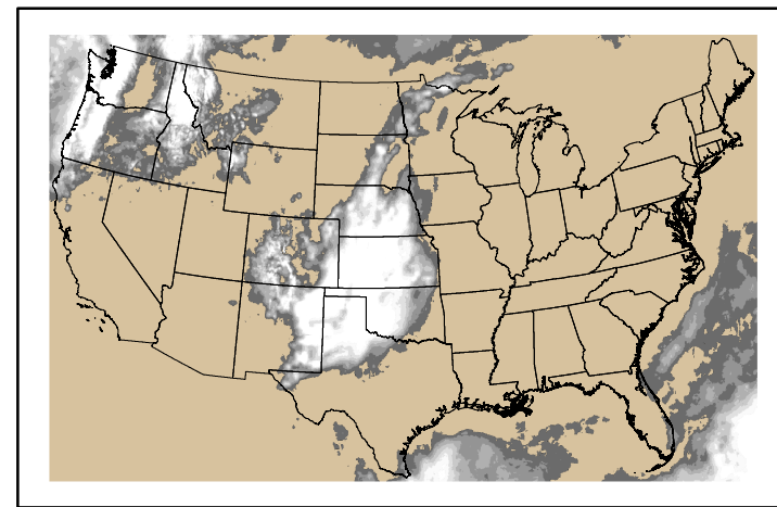
Precipitation p24m_2024101500f168.bil
