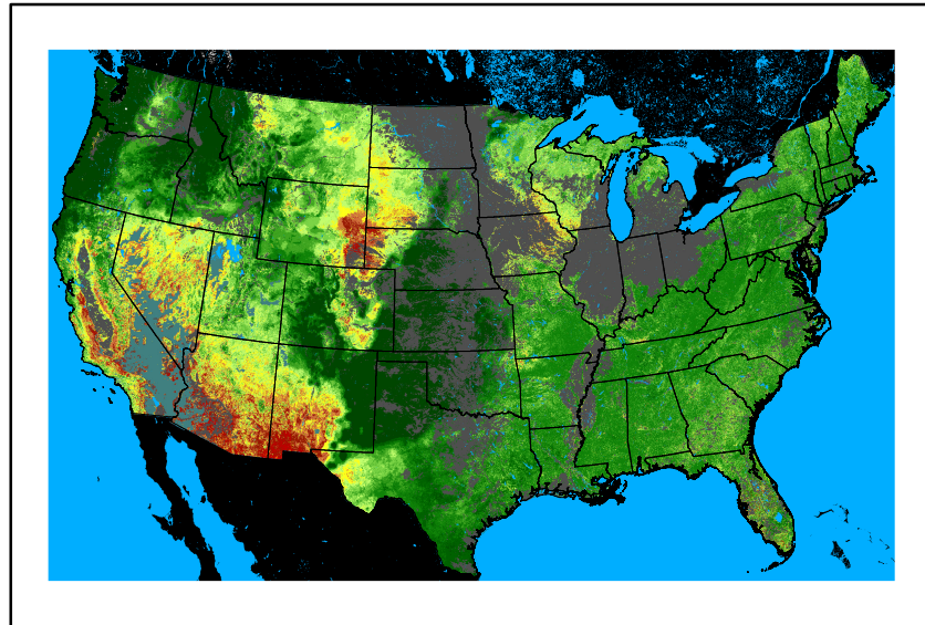
WFPI fp241021.bil
