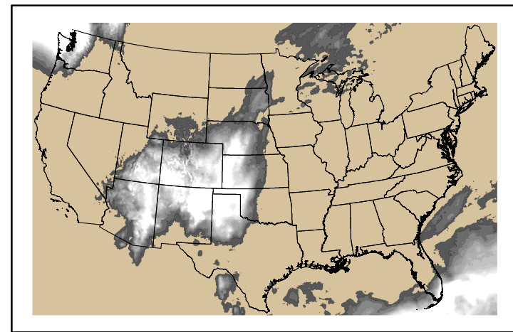
Precipitation p24m_2024101500f120.bil
