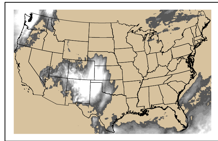
Precipitation p24m_2024101500f144.bil
