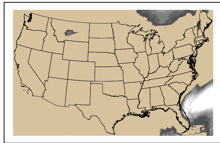
Precipitation p24m_2024101000f048.bil
