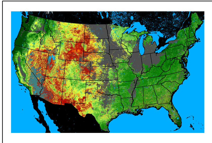
WFPI fp241016.bil
