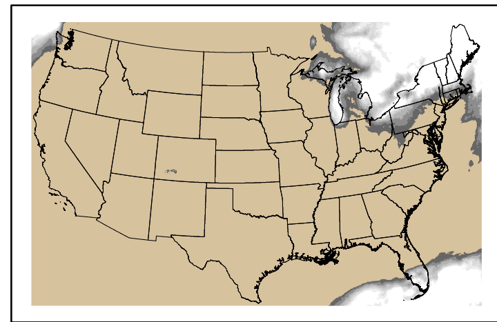
Precipitation p24m_2024101000f120.bil
