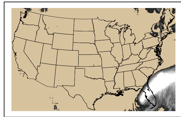
Precipitation p24m_2024101000f024.bil
