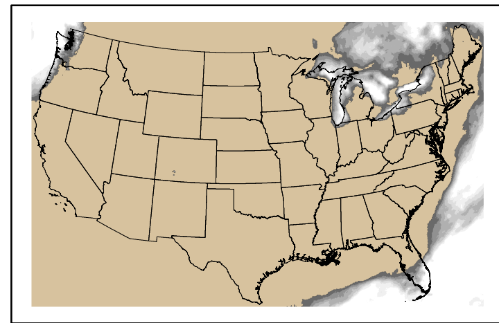
Precipitation p24m_2024101000f144.bil
