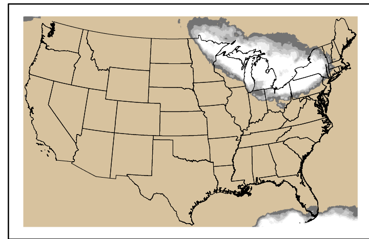
Precipitation p24m_2024101000f096.bil
