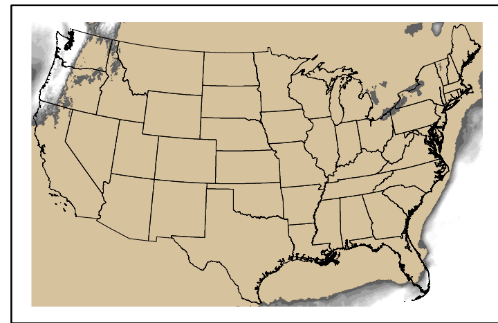
Precipitation p24m_2024101000f168.bil
