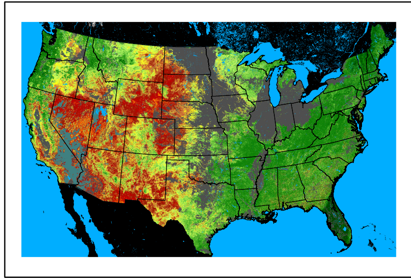
WFPI fp241010.bil
