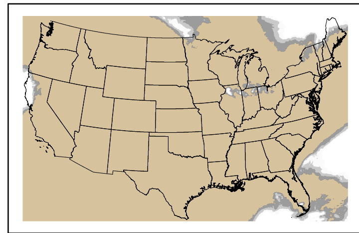
Precipitation p24m_2024101000f072.bil
