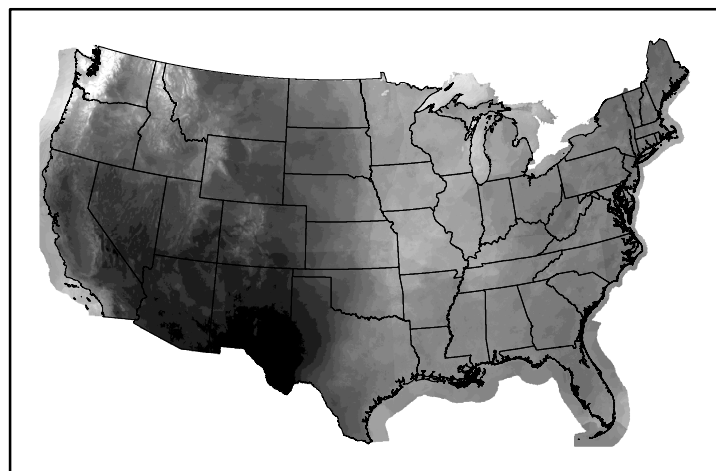
10hr Fuel Moisture mc10240604.bil
