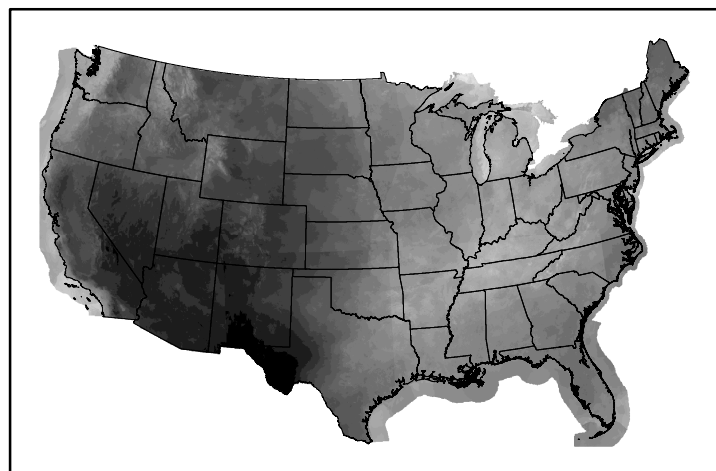
10hr Fuel Moisture mc10240605.bil
