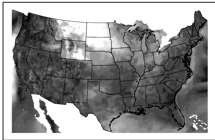
Wind Speed wspd20240605.bil
