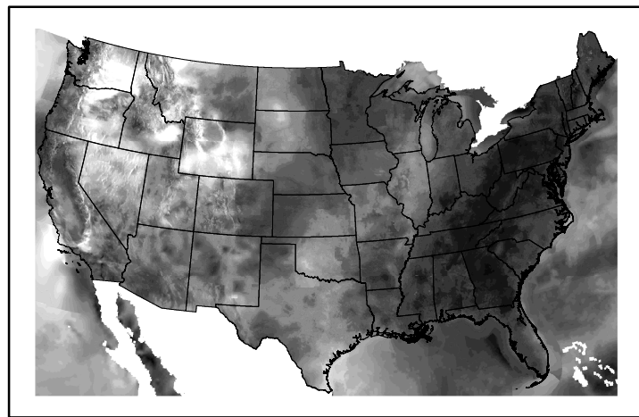
Wind Speed wspd20240603.bil
