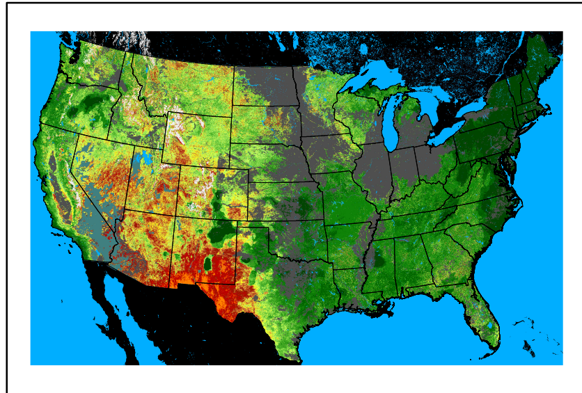
WFPI fp240607.bil
