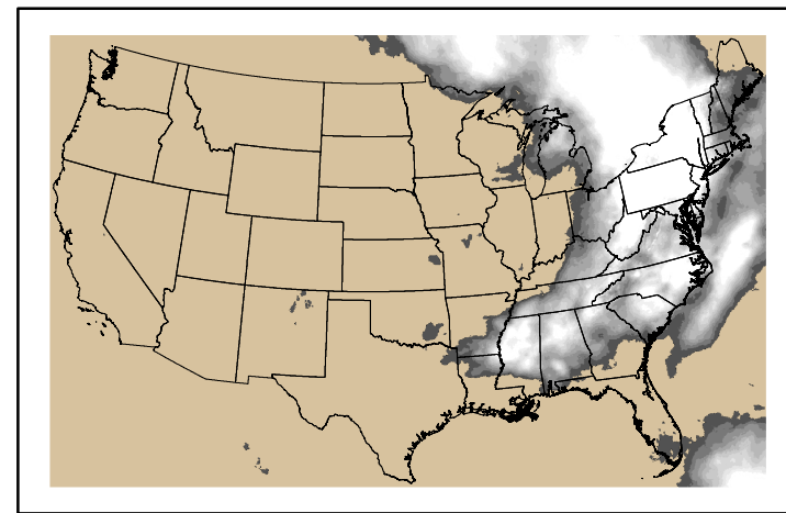
Precipitation p24m_2024060200f120.bil
