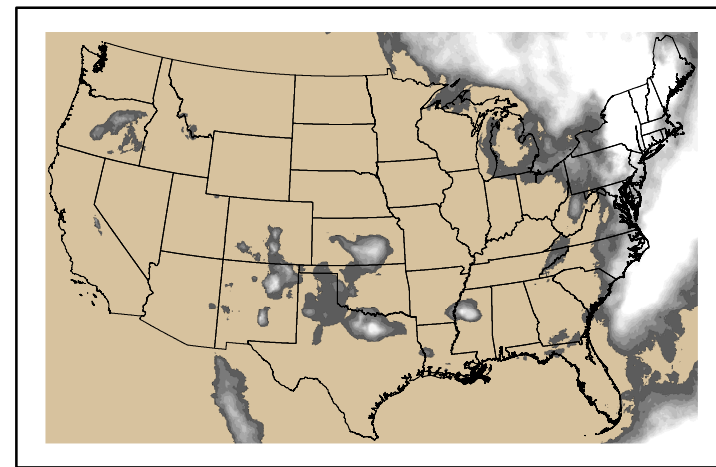
Precipitation p24m_2024060200f144.bil
