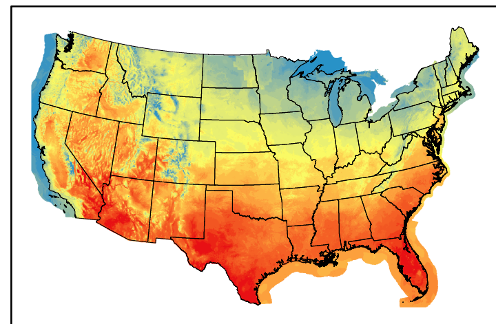
Dry Bulb Temp temp20240608.bil
