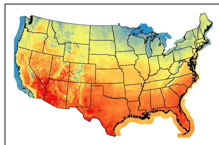
Dry Bulb Temp temp20240607.bil
