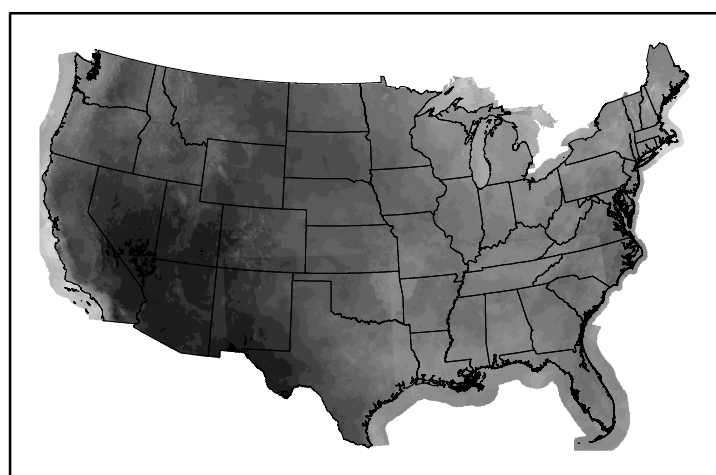
10hr Fuel Moisture mc10240607.bil
