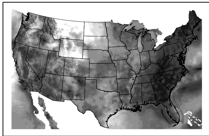
Wind Speed wspd20240604.bil
