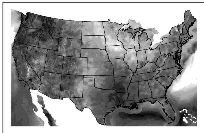
Wind Speed wspd20240607.bil
