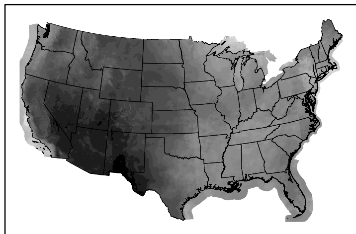
10hr Fuel Moisture mc10240606.bil
