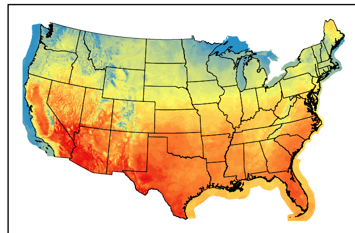
Dry Bulb Temp temp20240606.bil
