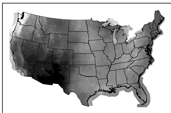
10hr Fuel Moisture mc10240602.bil
