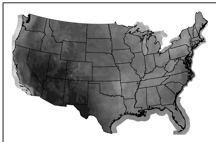
10hr Fuel Moisture mc10240608.bil
