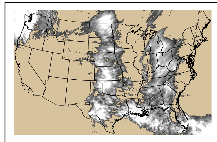
Precipitation p24m_2024060200f024.bil
