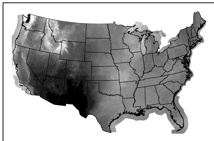
10hr Fuel Moisture mc10240603.bil
