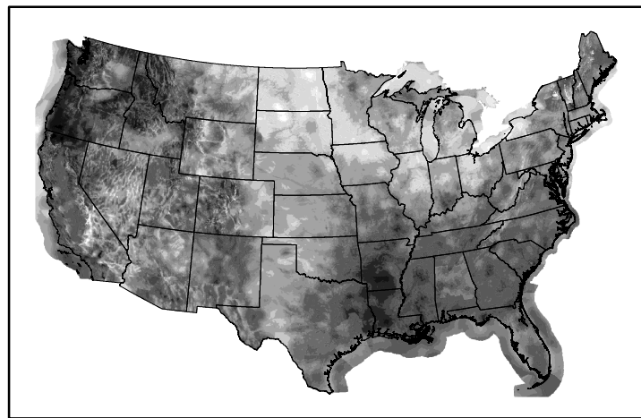
Wind Speed wspd20240608.bil
