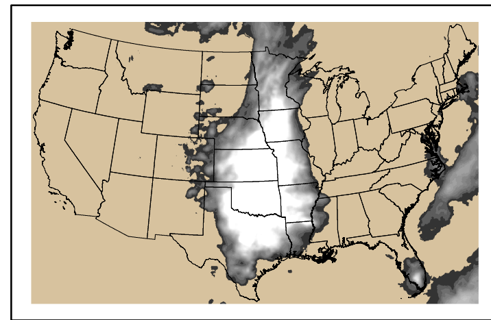
Precipitation p24m_2024052800f096.bil
