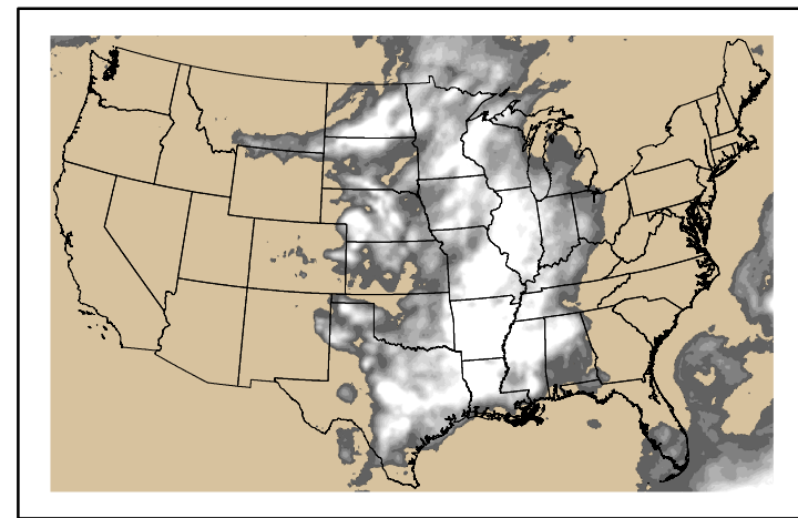
Precipitation p24m_2024052800f120.bil
