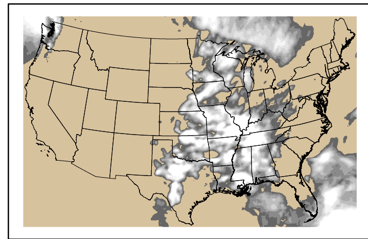
Precipitation p24m_2024052800f144.bil
