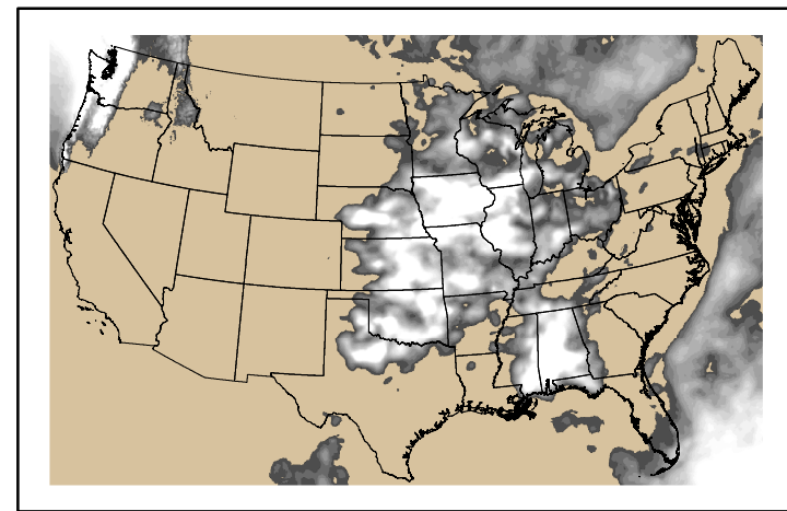
Precipitation p24m_2024052800f168.bil
