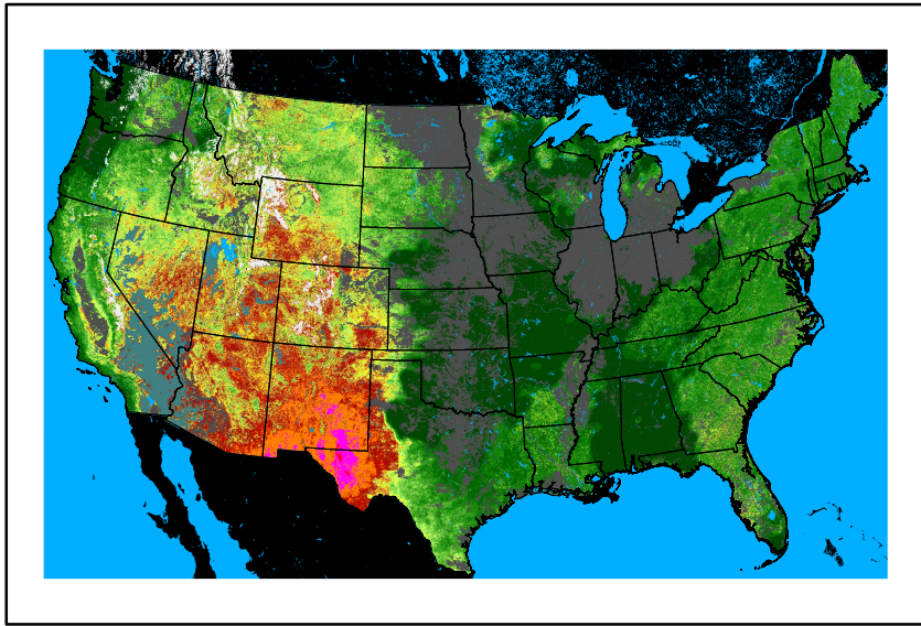
WFPI fp240603.bil
