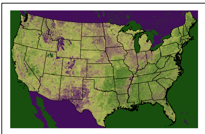
Greenness us24_141147wk_greenness.img
