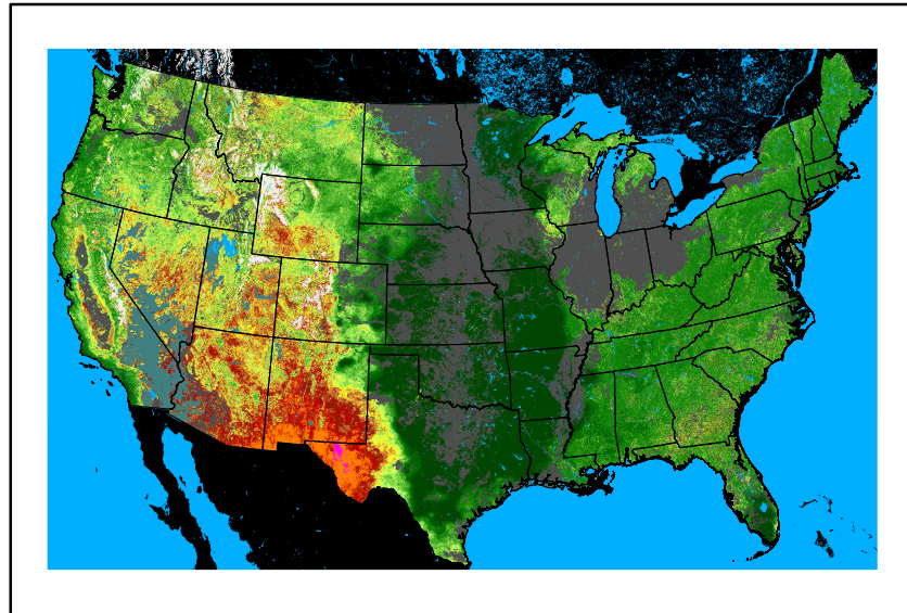
WFPI fp240531.bil
