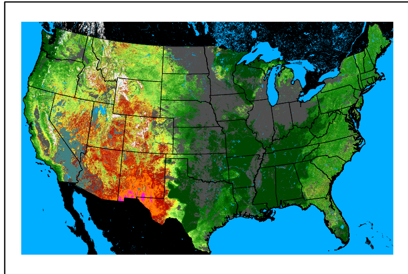
WFPI fp240602.bil
