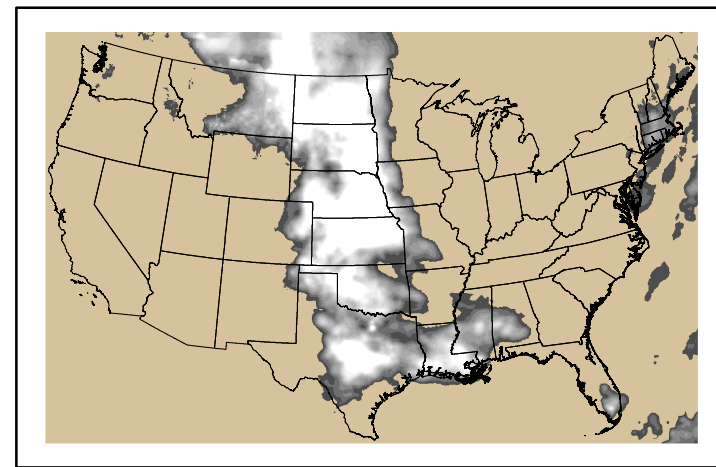
Precipitation p24m_2024052800f072.bil
