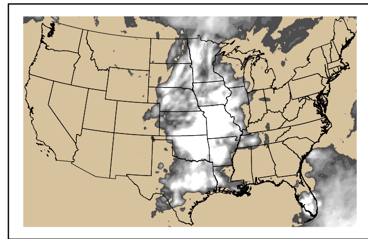
Precipitation p24m_2024052600f168.bil
