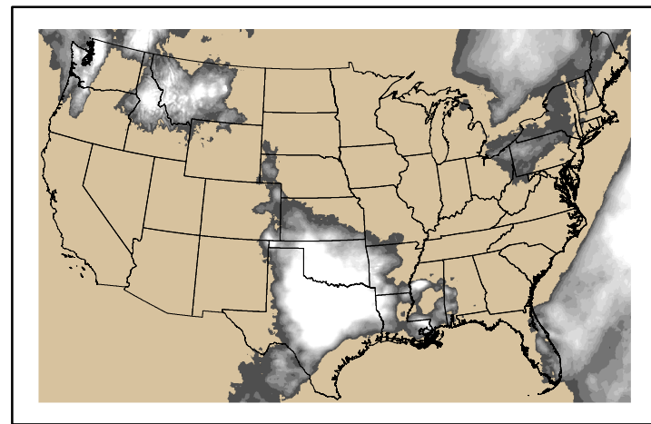
Precipitation p24m_2024052600f096.bil
