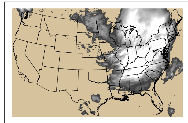
Precipitation p24m_2024052600f048.bil
