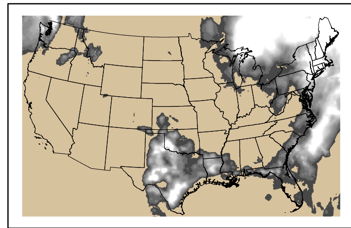
Precipitation p24m_2024052600f072.bil
