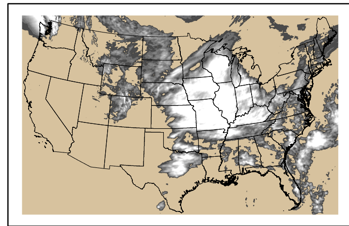
Precipitation p24m_2024052600f024.bil
