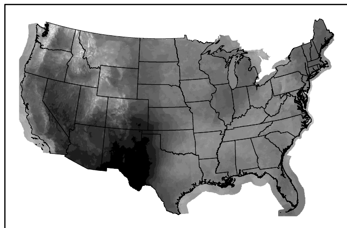
10hr Fuel Moisture mc10240525.bil
