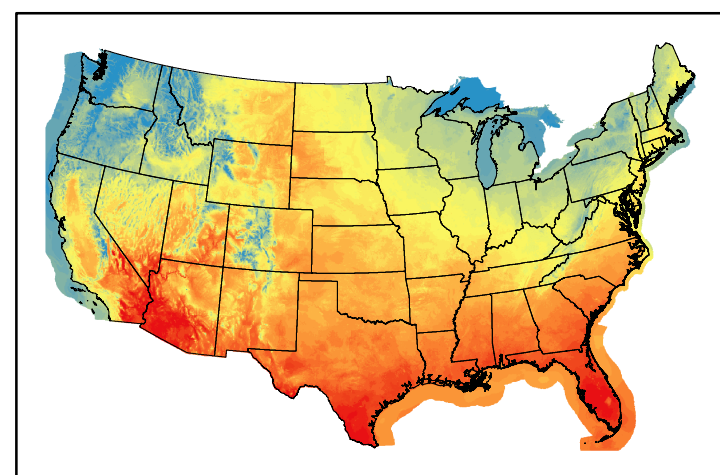
Dry Bulb Temp temp20240529.bil
