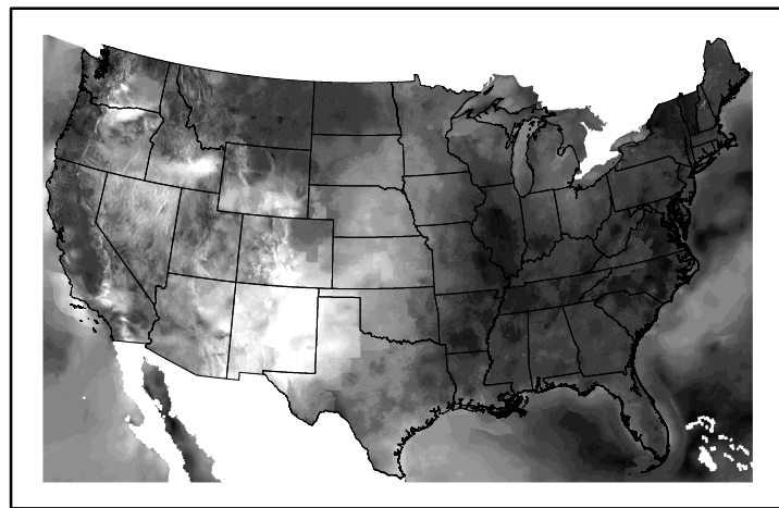
Wind Speed wspd20240525.bil
