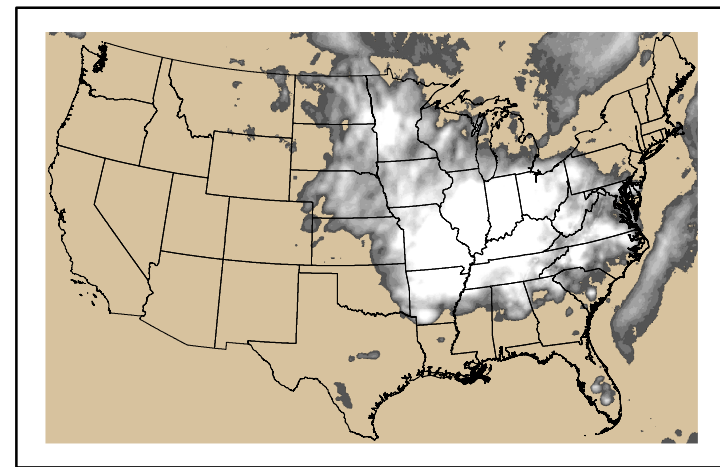
Precipitation p24m_2024052100f168.bil
