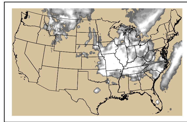
Precipitation p24m_2024052100f144.bil
