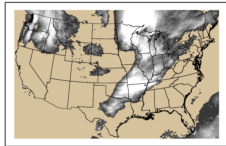
Precipitation p24m_2024052100f048.bil
