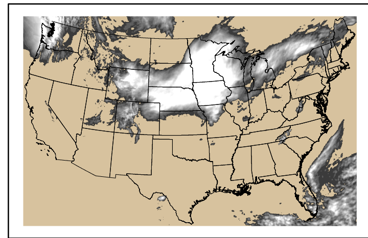
Precipitation p24m_2024052100f024.bil
