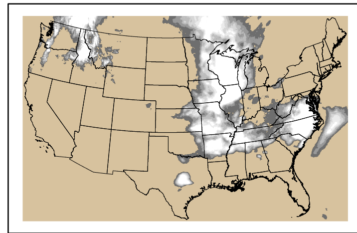
Precipitation p24m_2024052100f120.bil
