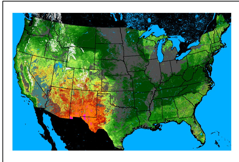
WFPI fp240524.bil
