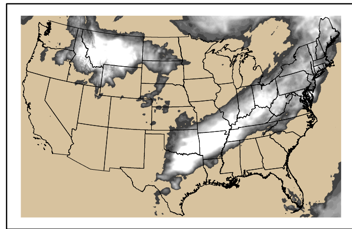
Precipitation p24m_2024052100f072.bil
