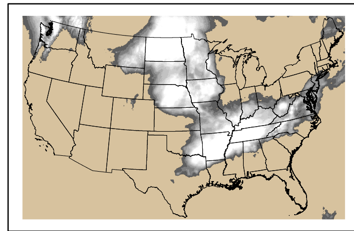
Precipitation p24m_2024052100f096.bil
