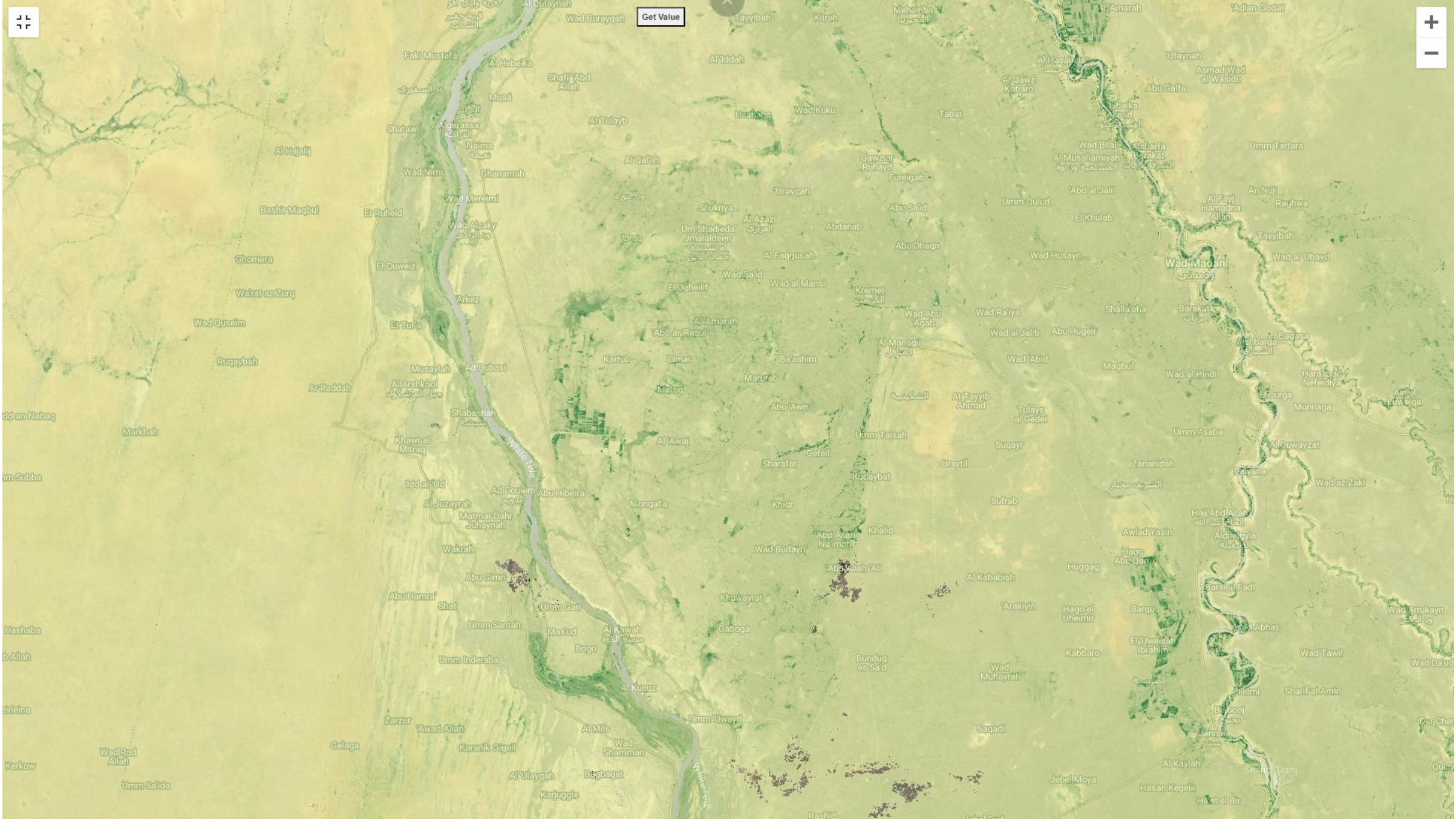
Sentinel 2 Maximum NDVI : June 16 - 30, 2023
