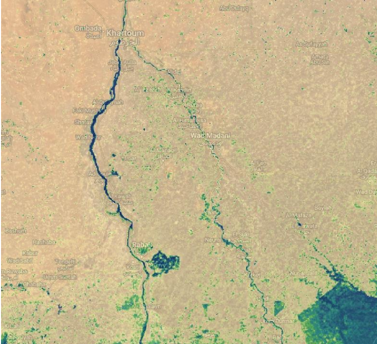
SSEBop VIIRS v6 July Dekad 3, 2023
