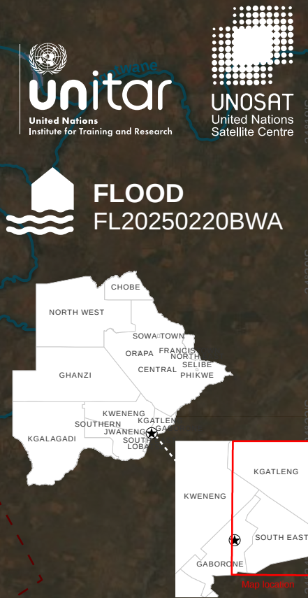
Satellite detected water extents in Gaborone, South East and Kgatleng Districts, Botswana as of 23 to 25 February 2025
