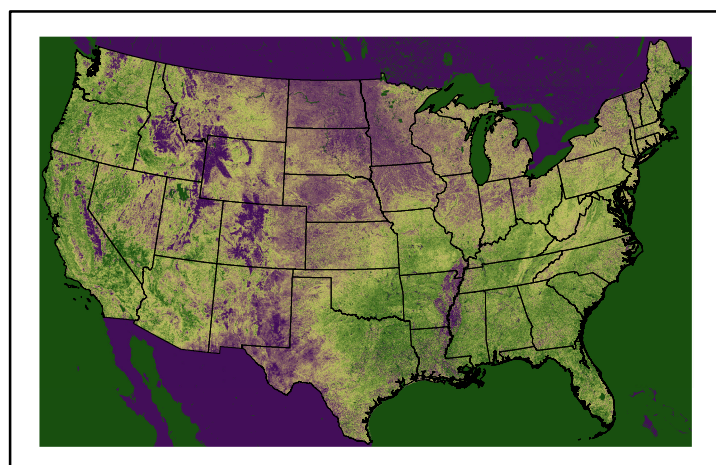
Greenness us24_106112wk_greenness.img
