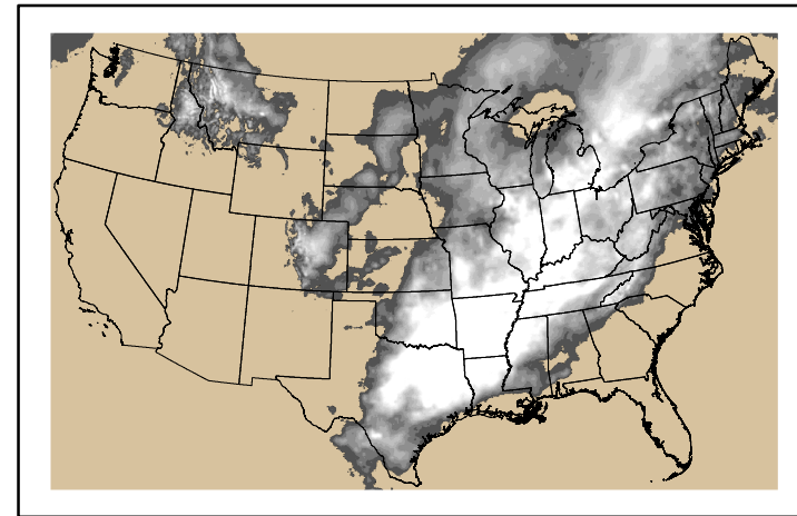
Precipitation p24m_2024042800f144.bil
