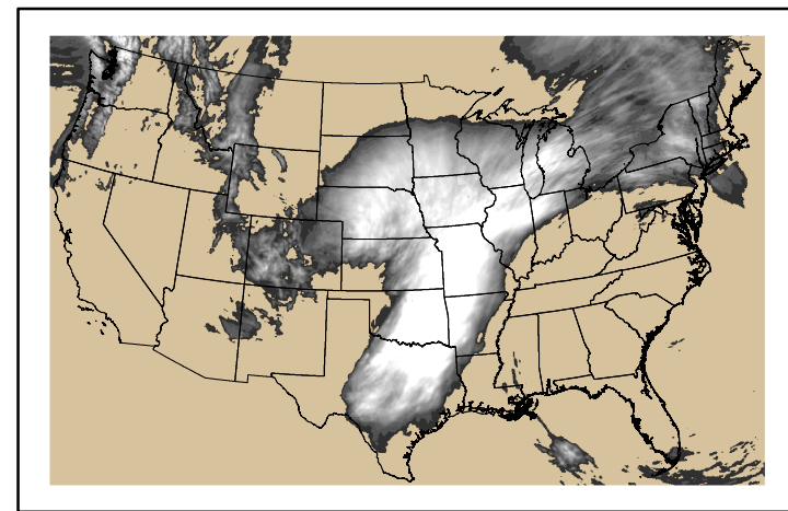
Precipitation p24m_2024042800f024.bil
