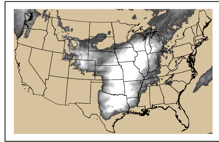
Precipitation p24m_2024042800f120.bil
