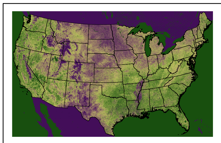
Greenness us24_106112wk_greenness.img
