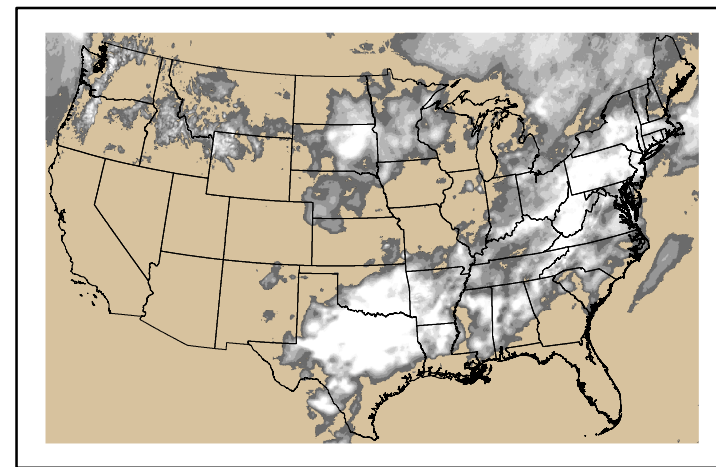
Precipitation p24m_2024042800f168.bil
