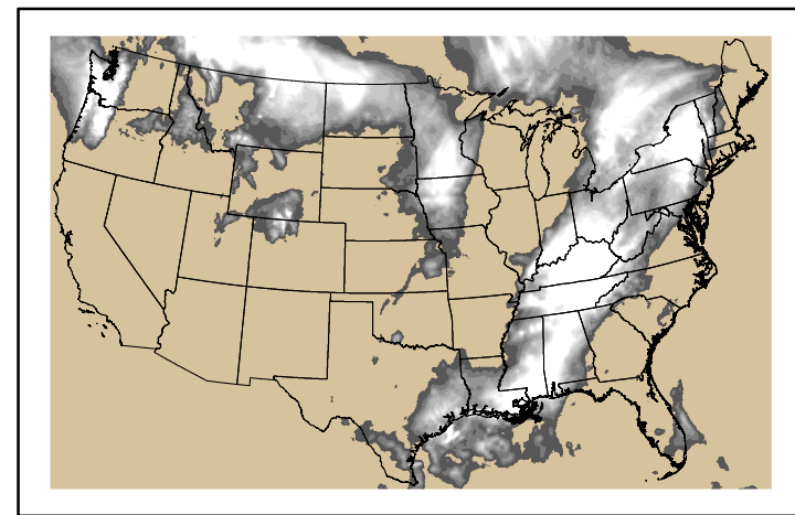
Precipitation p24m_2024042800f072.bil
