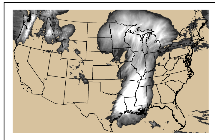
Precipitation p24m_2024042800f048.bil
