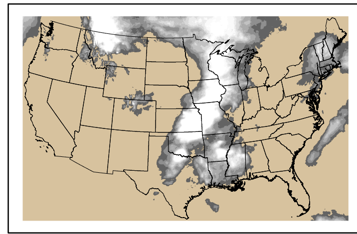
Precipitation p24m_2024042800f096.bil
