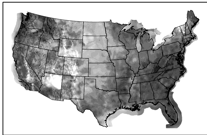
Wind Speed wspd20240524.bil
