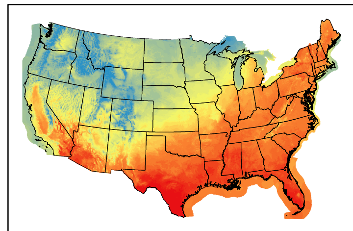
Dry Bulb Temp temp20240522.bil
