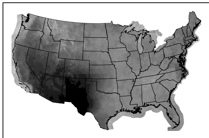
10hr Fuel Moisture mc10240524.bil
