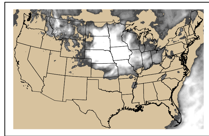
Precipitation p24m_2024051500f168.bil
