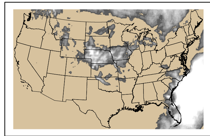
Precipitation p24m_2024051500f144.bil
