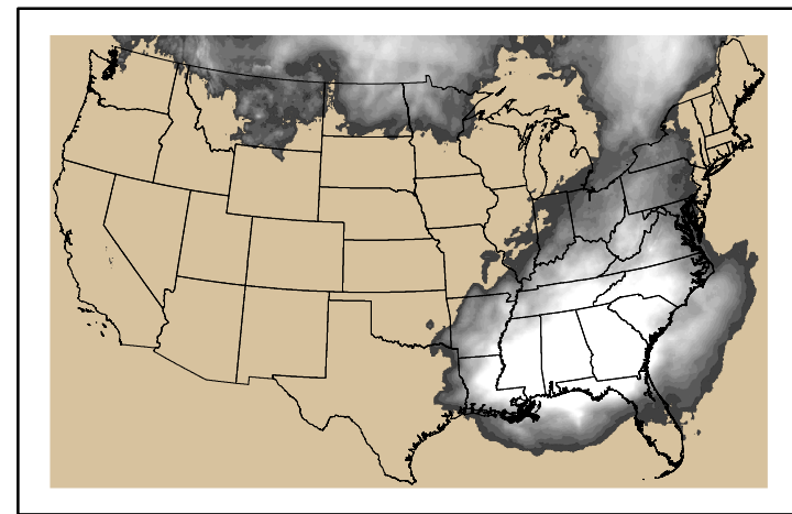
Precipitation p24m_2024051500f096.bil
