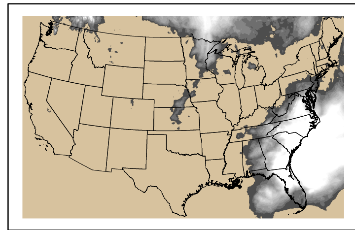
Precipitation p24m_2024051500f120.bil
