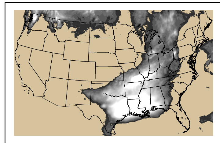
Precipitation p24m_2024051500f072.bil
