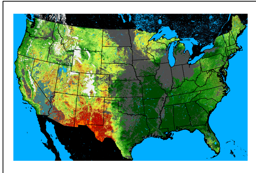
WFPI fp240513.bil
