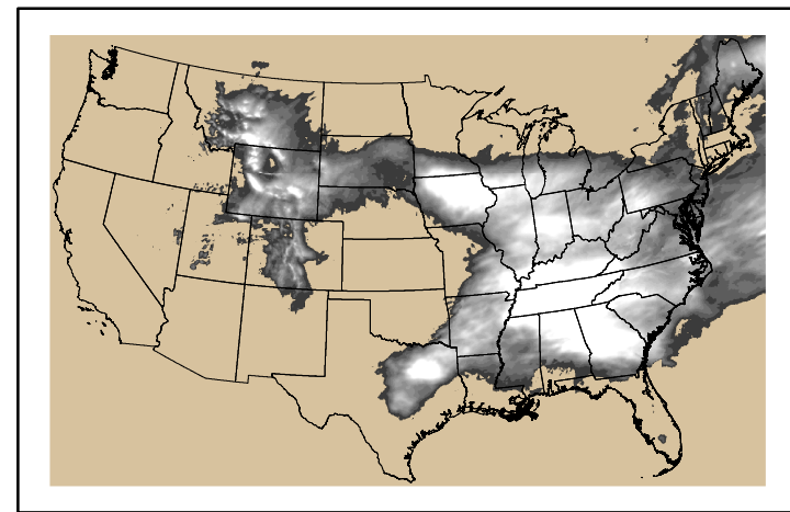
Precipitation p24m_2024050900f024.bil
