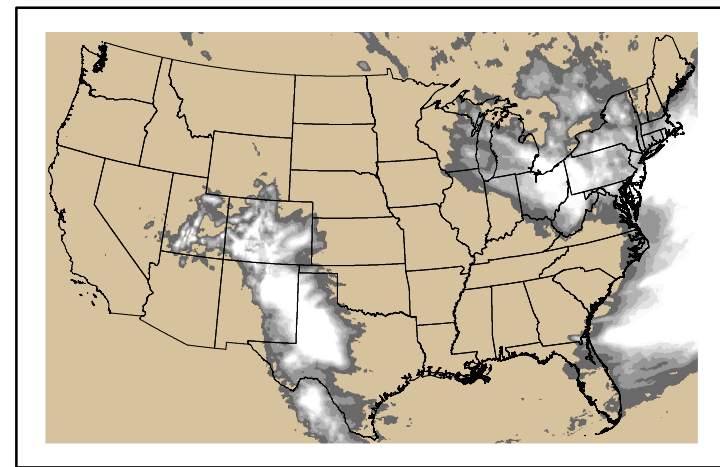
Precipitation p24m_2024050900f072.bil
