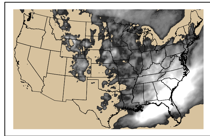
Precipitation p24m_2024050900f168.bil
