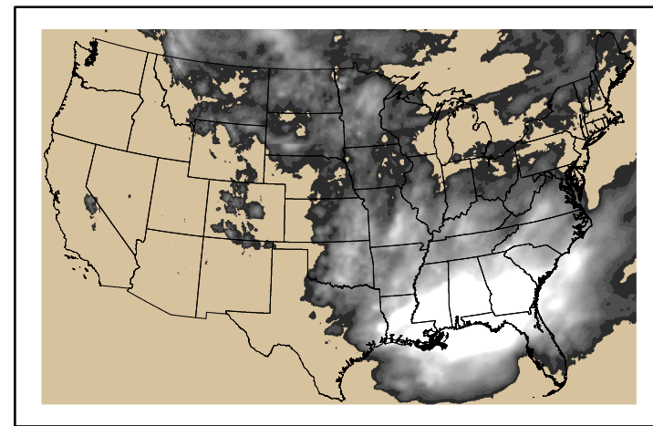
Precipitation p24m_2024050900f144.bil
