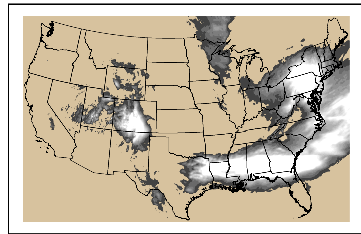
Precipitation p24m_2024050900f048.bil
