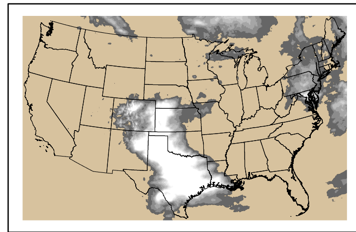
Precipitation p24m_2024050900f096.bil
