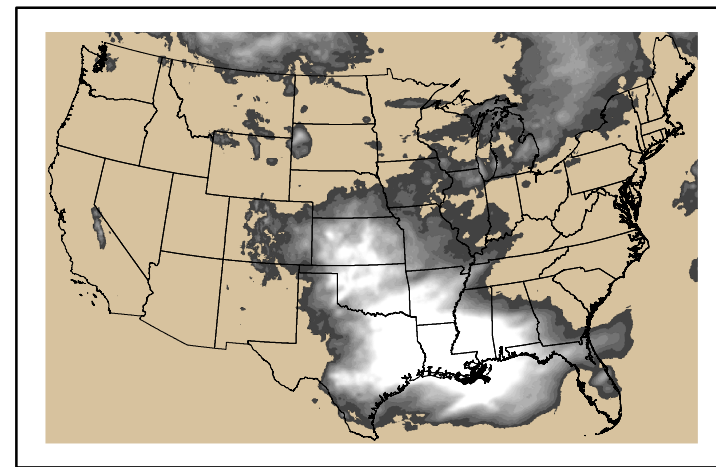
Precipitation p24m_2024050900f120.bil
