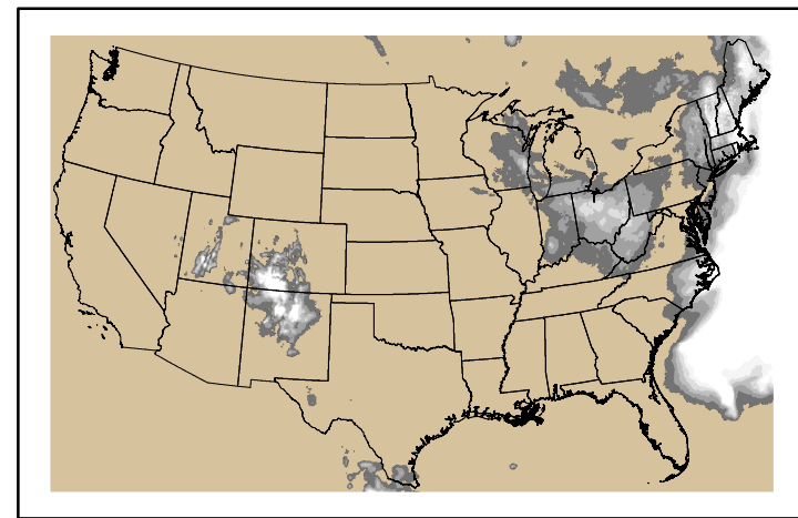
Precipitation p24m_2024050800f096.bil
