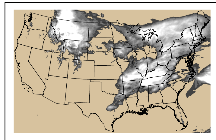
Precipitation p24m_2024050800f024.bil
