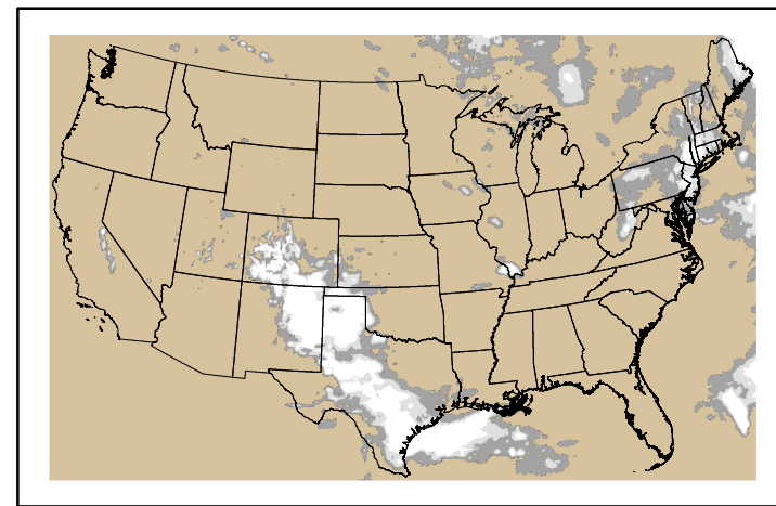
Precipitation p24m_2024050800f120.bil
