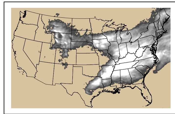
Precipitation p24m_2024050800f048.bil
