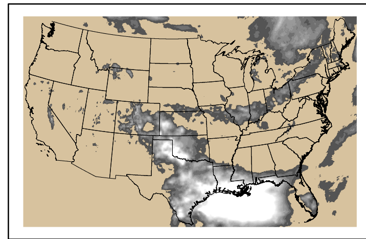
Precipitation p24m_2024050800f144.bil
