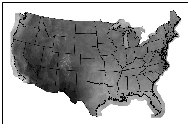
10hr Fuel Moisture mc10240514.bil
