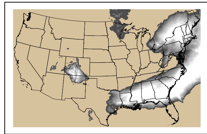
Precipitation p24m_2024050700f096.bil
