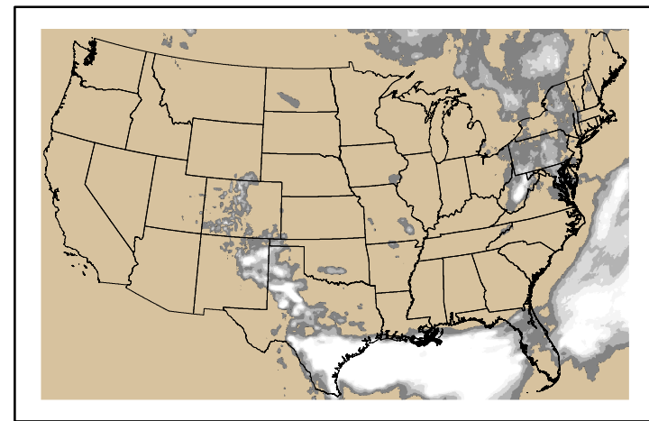
Precipitation p24m_2024050700f144.bil
