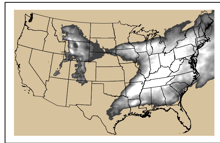
Precipitation p24m_2024050700f072.bil
