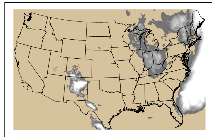
Precipitation p24m_2024050700f120.bil
