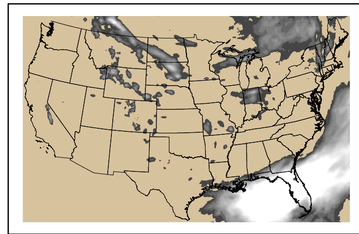
Precipitation p24m_2024050700f168.bil
