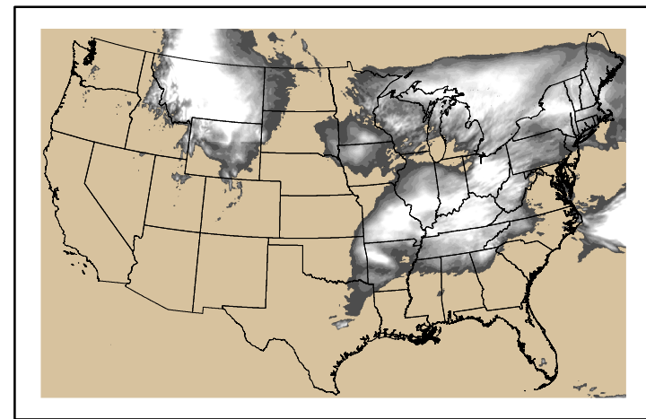
Precipitation p24m_2024050700f048.bil
