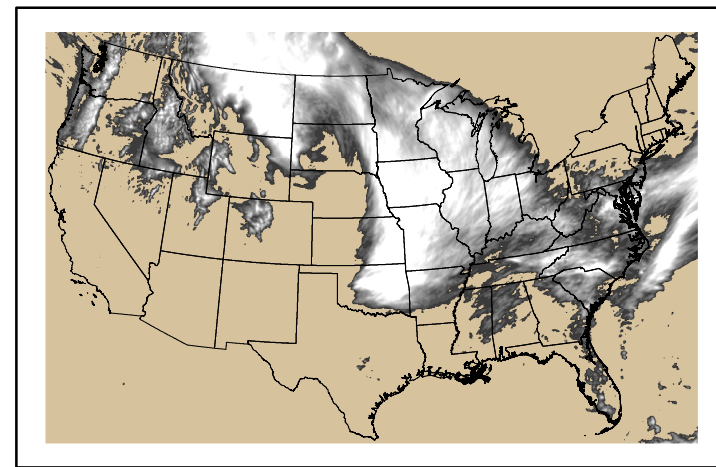
Precipitation p24m_2024050700f024.bil
