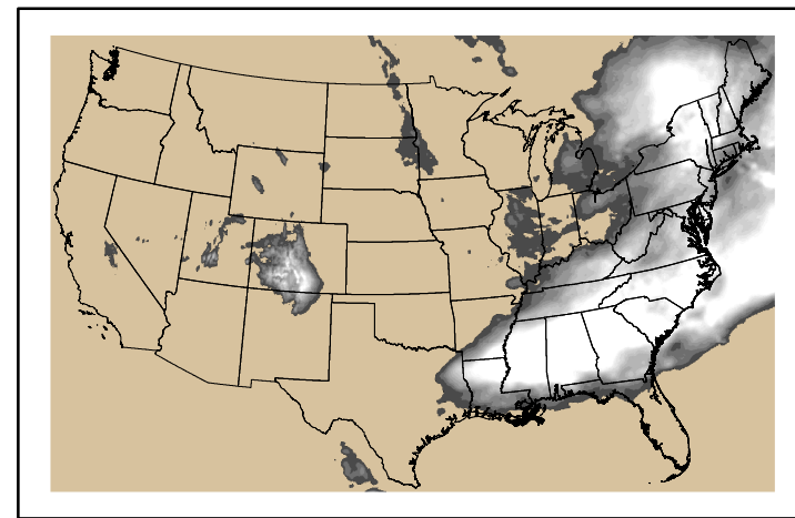
Precipitation p24m_2024050600f120.bil
