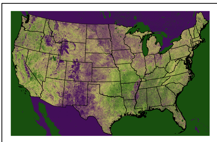
Greenness us24_120126wk_greenness.img
