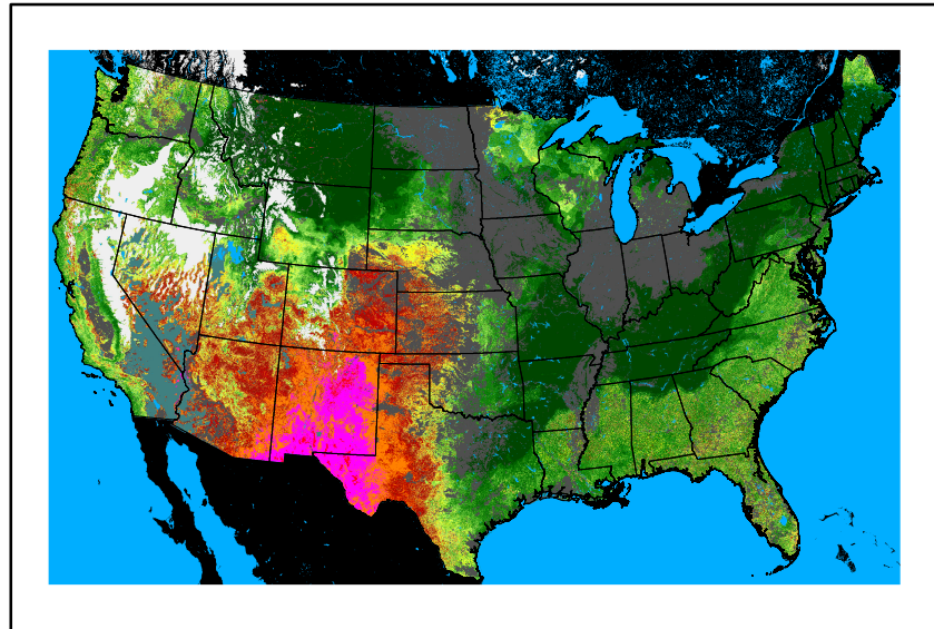
WFPI fp240508.bil
