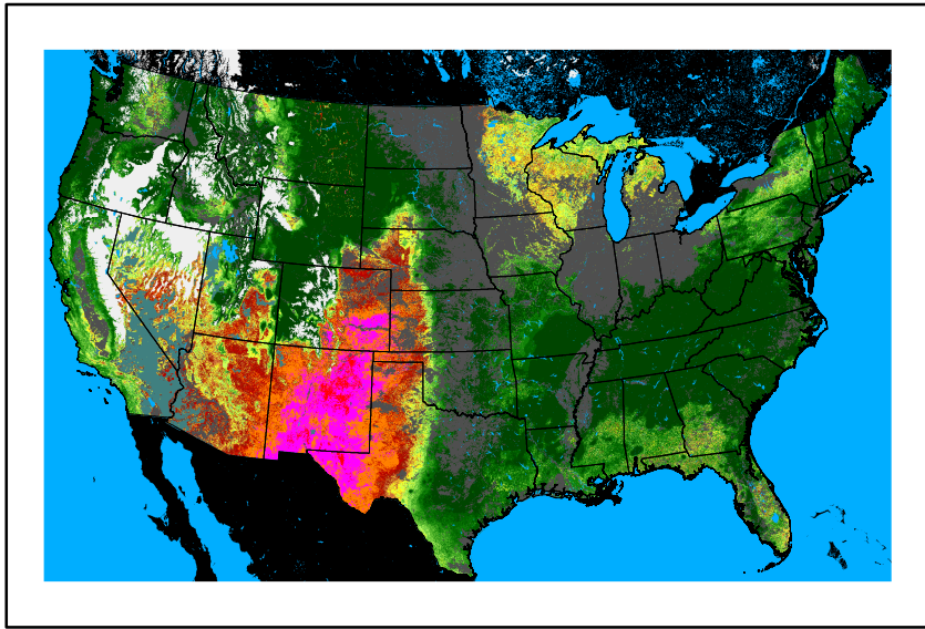
WFPI fp240506.bil
