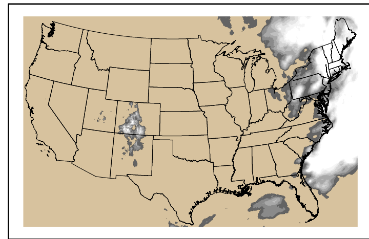
Precipitation p24m_2024050600f144.bil
