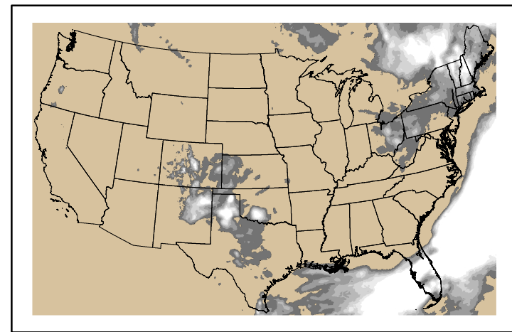
Precipitation p24m_2024050600f168.bil
