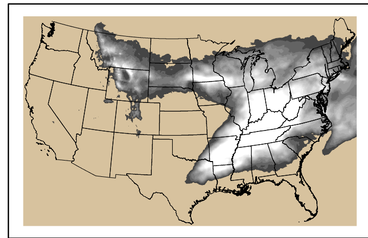
Precipitation p24m_2024050600f096.bil
