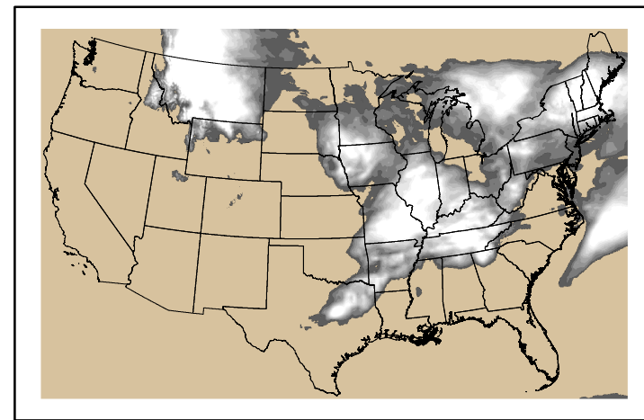
Precipitation p24m_2024050600f072.bil
