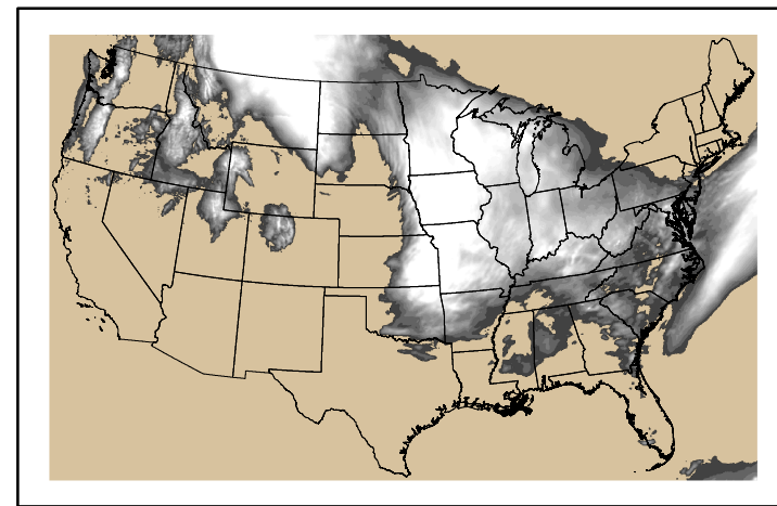
Precipitation p24m_2024050600f048.bil
