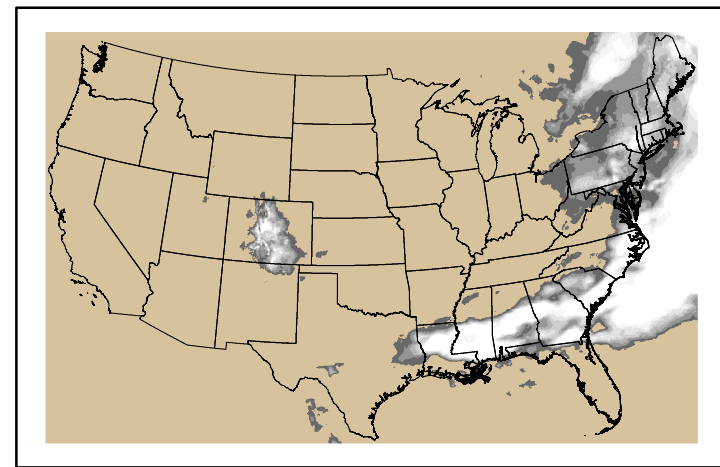
Precipitation p24m_2024050500f168.bil
