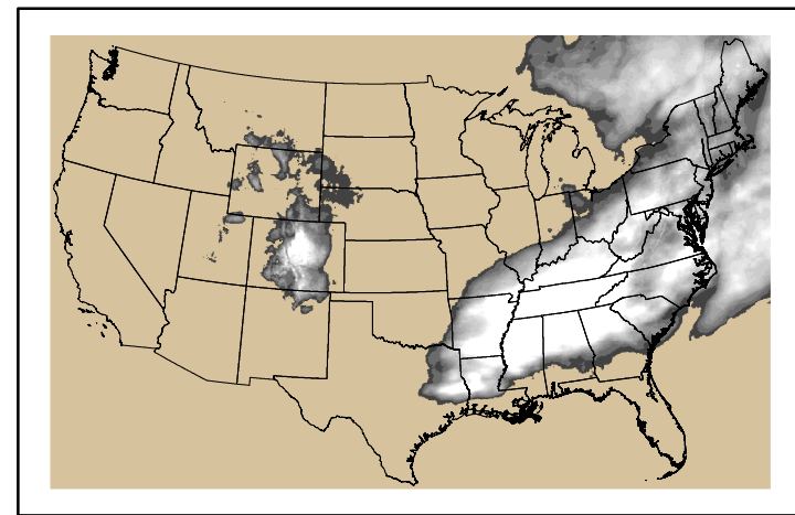
Precipitation p24m_2024050500f144.bil
