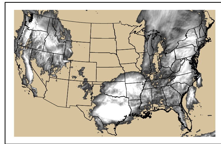
Precipitation p24m_2024050500f024.bil
