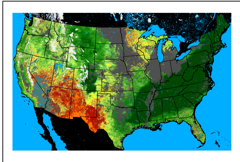
WFPI fp240510.bil
