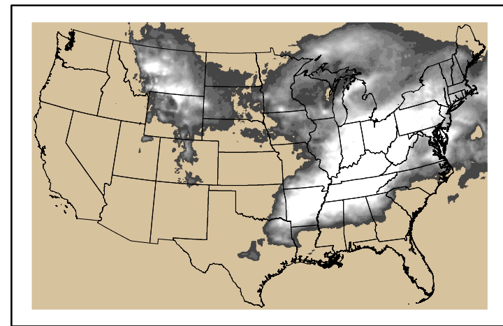
Precipitation p24m_2024050500f120.bil
