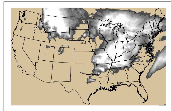
Precipitation p24m_2024050500f096.bil
