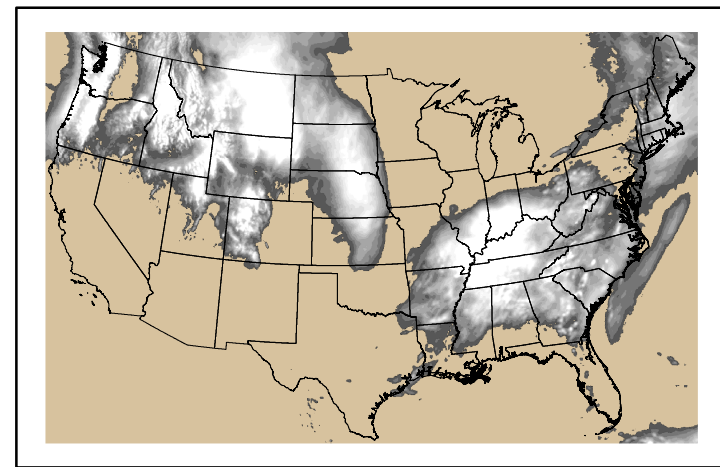
Precipitation p24m_2024050500f048.bil
