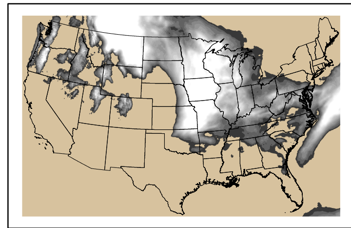
Precipitation p24m_2024050500f072.bil
