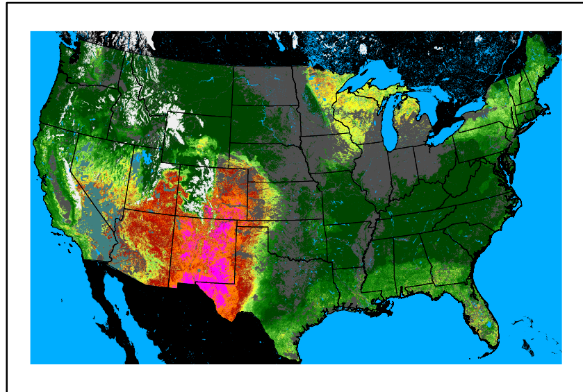
WFPI fp240506.bil
