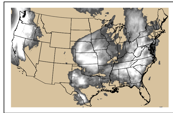
Precipitation p24m_2024050100f096.bil
