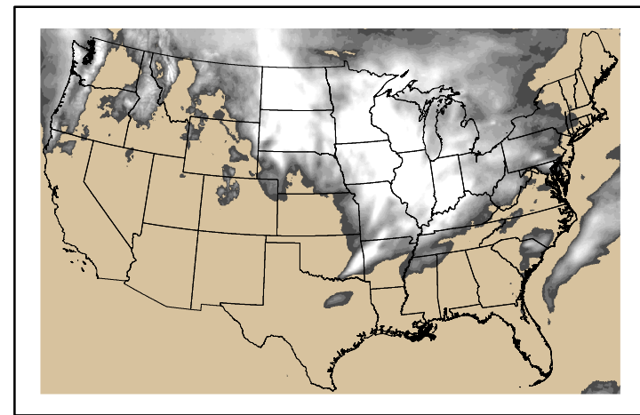
Precipitation p24m_2024050100f168.bil
