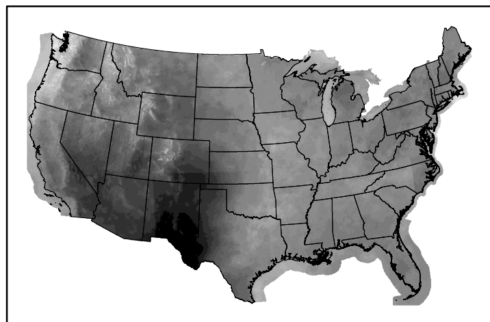
10hr Fuel Moisture mc10240506.bil
