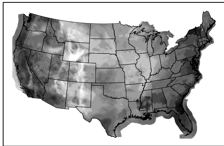
Wind Speed wspd20240507.bil
