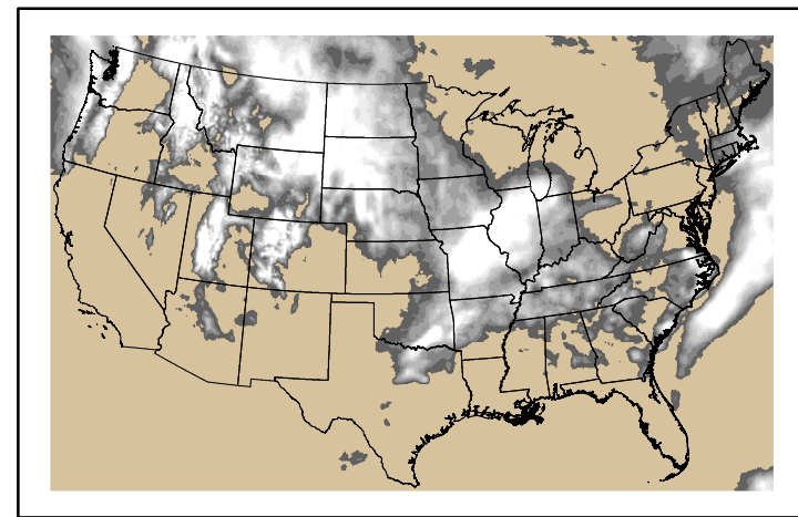
Precipitation p24m_2024050100f144.bil
