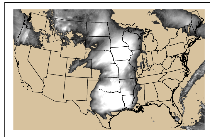
Precipitation p24m_2024050100f048.bil
