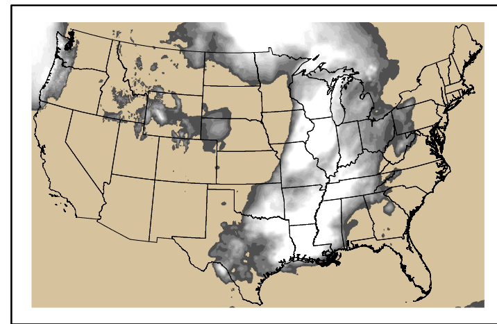
Precipitation p24m_2024050100f072.bil
