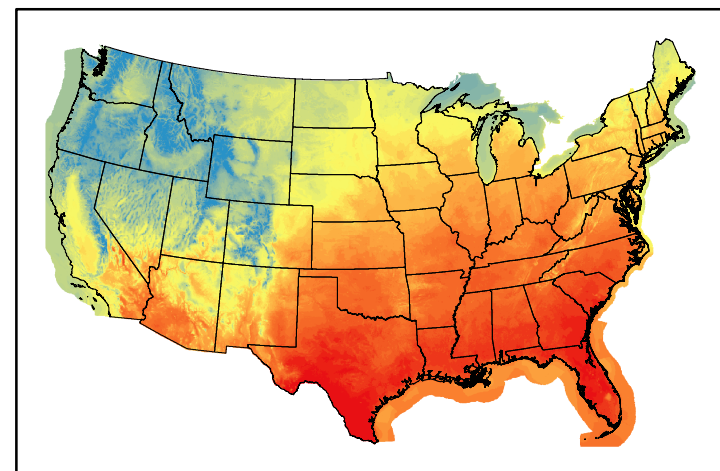
Dry Bulb Temp temp20240507.bil
