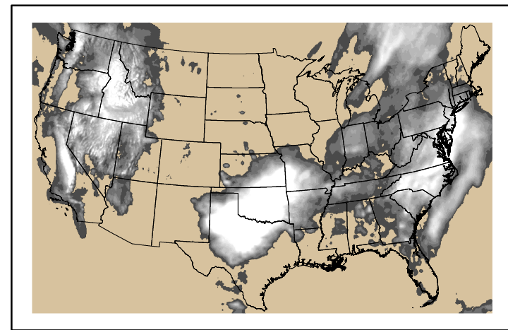
Precipitation p24m_2024050100f120.bil
