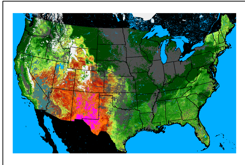
WFPI fp240507.bil
