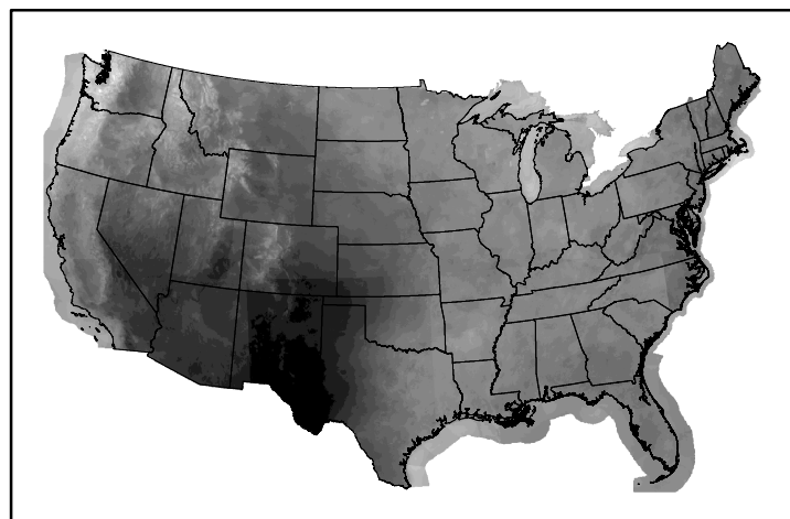
10hr Fuel Moisture mc10240507.bil
