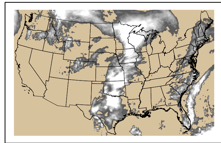
Precipitation p24m_2024050100f024.bil
