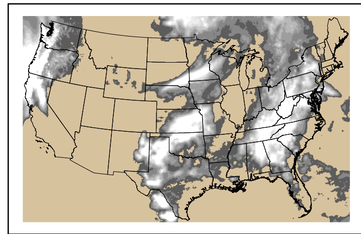
Precipitation p24m_2024043000f120.bil
