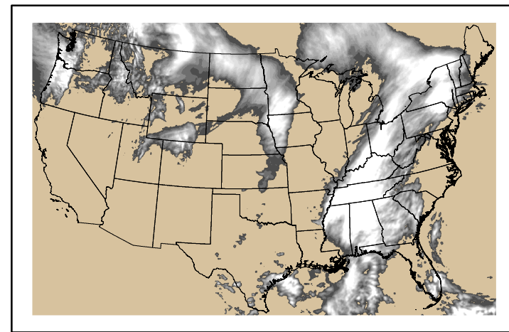
Precipitation p24m_2024043000f024.bil
