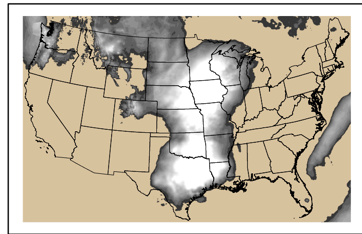
Precipitation p24m_2024043000f072.bil
