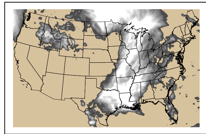
Precipitation p24m_2024043000f096.bil
