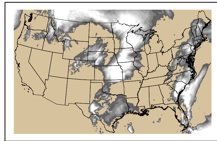
Precipitation p24m_2024043000f048.bil
