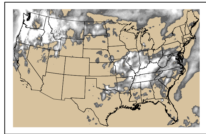
Precipitation p24m_2024043000f168.bil
