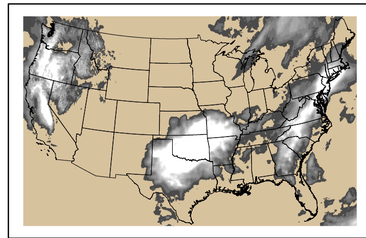
Precipitation p24m_2024043000f144.bil
