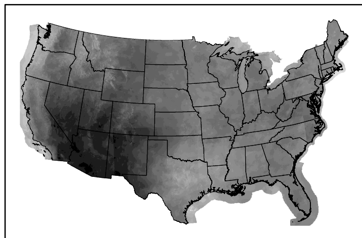
10hr Fuel Moisture mc10240505.bil
