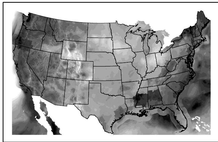
Wind Speed wspd20240503.bil
