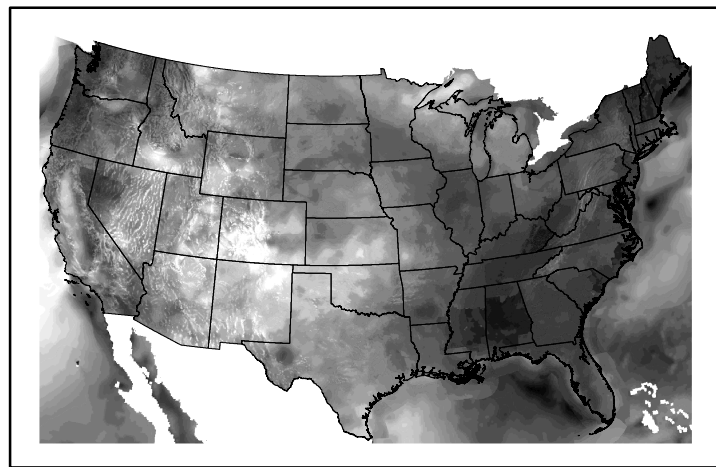
Wind Speed wspd20240501.bil
