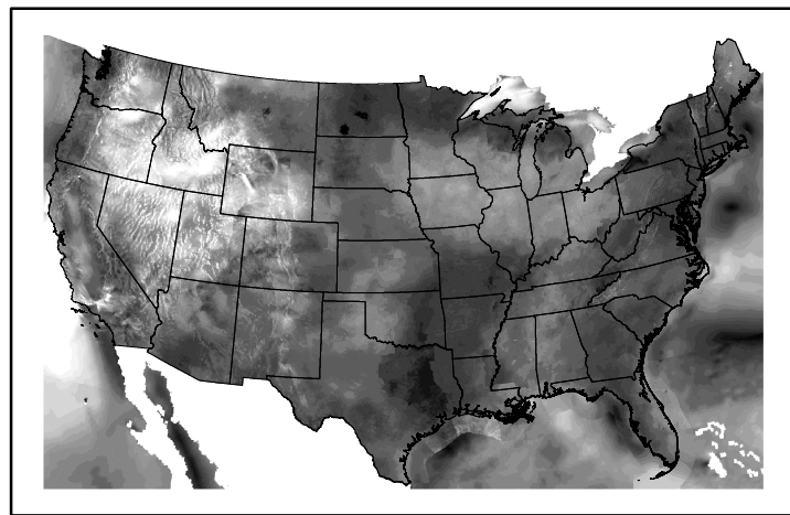
Wind Speed wspd20240429.bil
