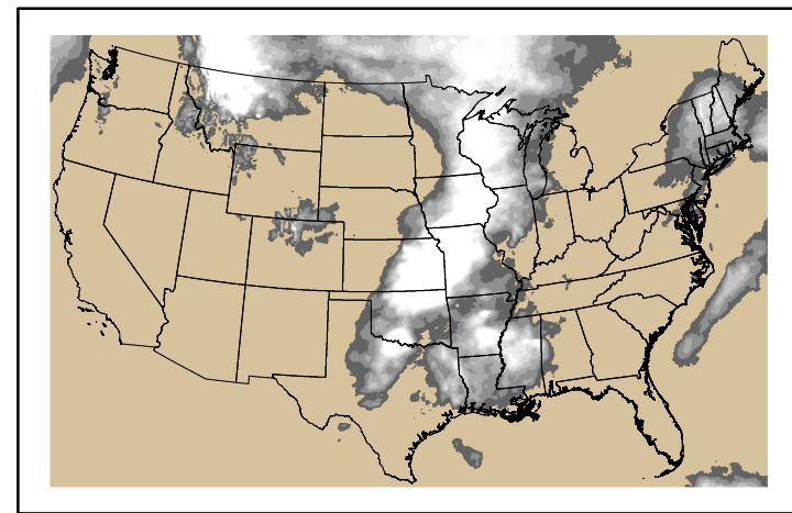
Precipitation p24m_2024042800f096.bil
