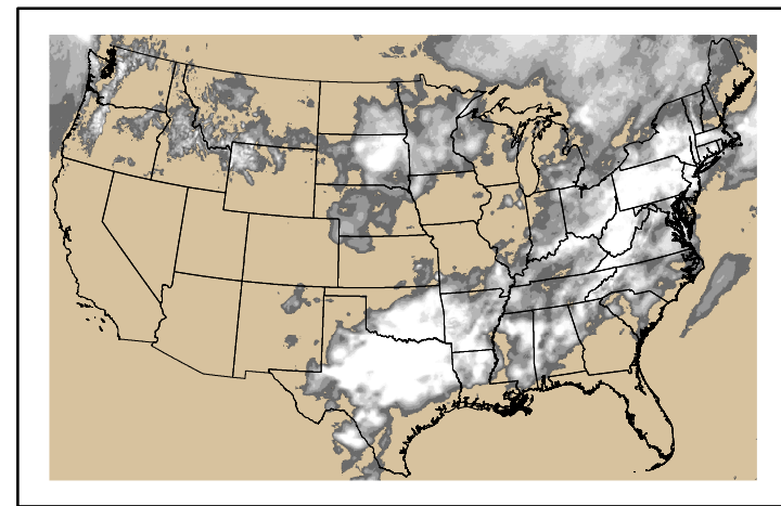
Precipitation p24m_2024042800f168.bil
