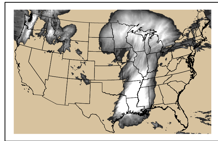
Precipitation p24m_2024042800f048.bil
