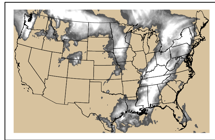
Precipitation p24m_2024042800f072.bil
