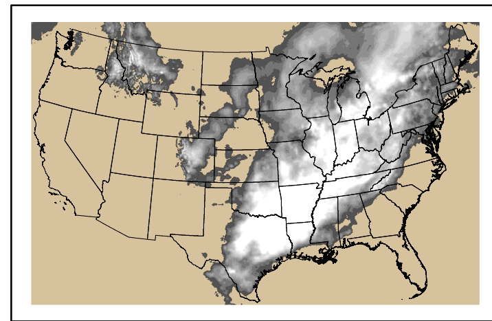
Precipitation p24m_2024042800f144.bil
