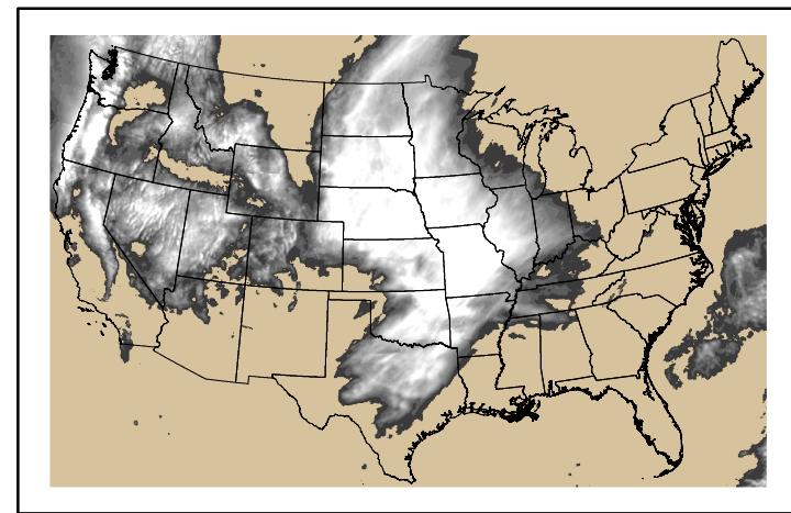
Precipitation p24m_2024042600f024.bil
