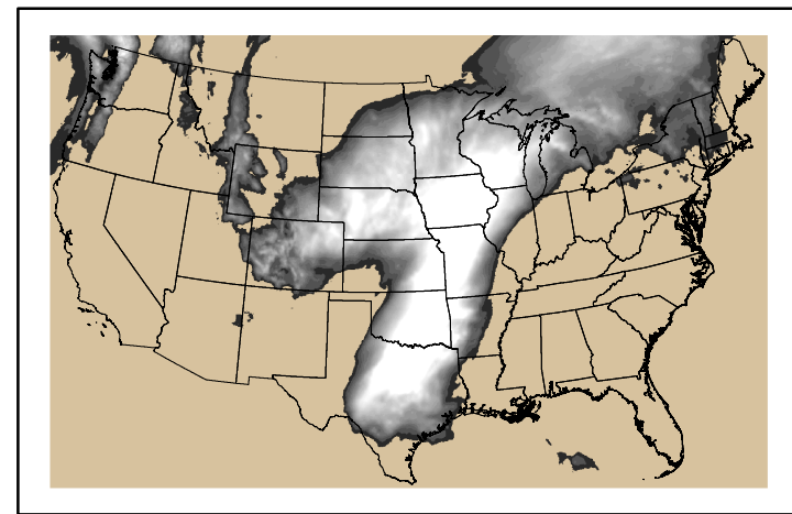
Precipitation p24m_2024042600f072.bil
