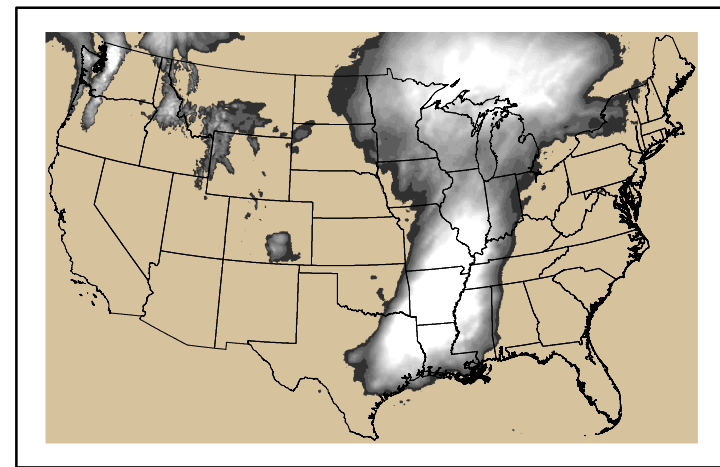
Precipitation p24m_2024042600f096.bil
