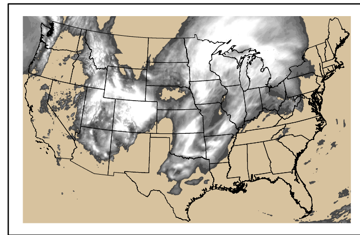
Precipitation p24m_2024042600f048.bil
