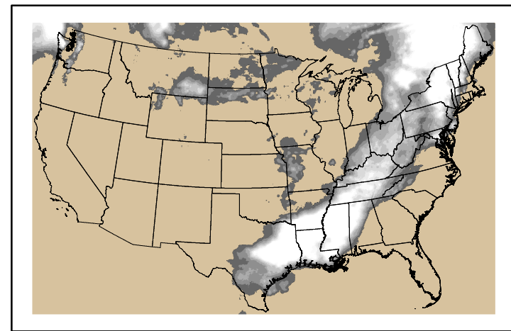
Precipitation p24m_2024042600f120.bil
