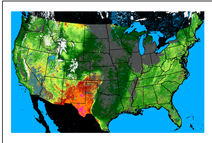
WFPI fp240428.bil
