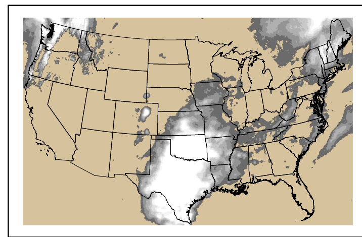
Precipitation p24m_2024042600f168.bil
