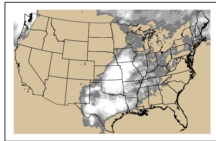
Precipitation p24m_2024042600f144.bil
