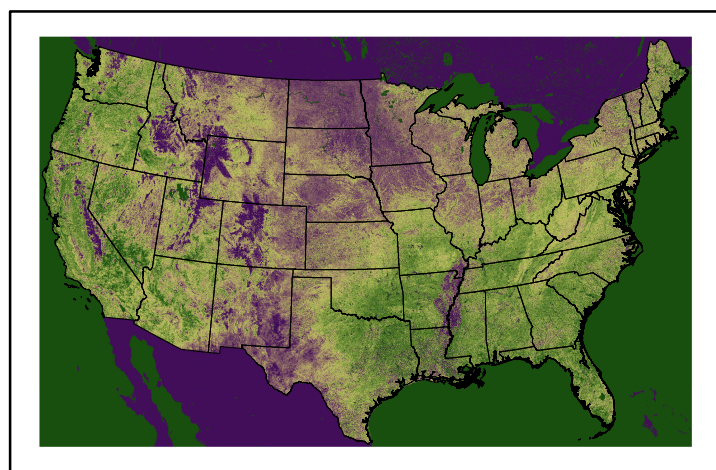
Greenness us24_106112wk_greenness.img
