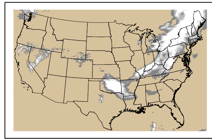
Precipitation p24m_2024042400f024.bil
