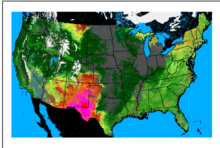
WFPI fp240426.bil
