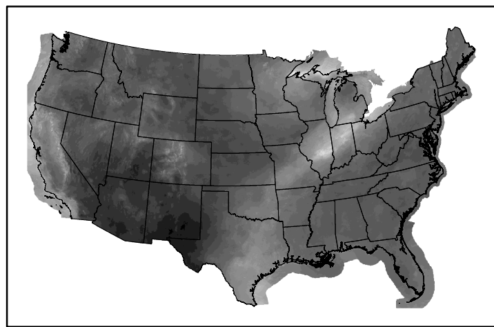
10hr Fuel Moisture mc10240423.bil
