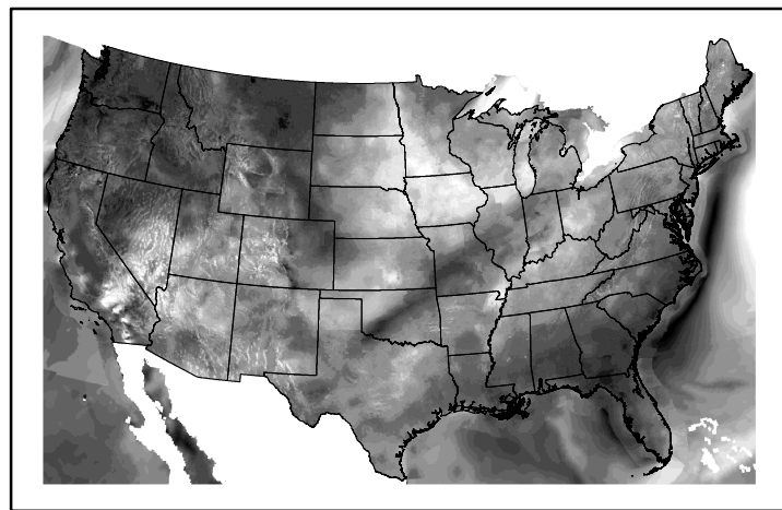
Wind Speed wspd20240423.bil
