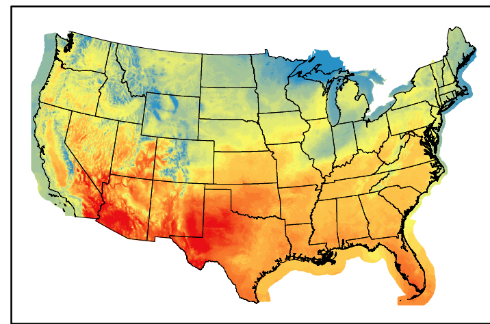
Dry Bulb Temp temp20240423.bil
